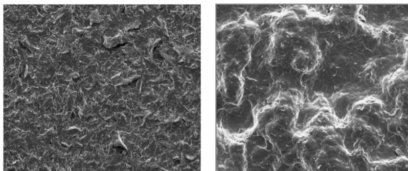
Figure 11. Nano- and microtextured surfaces visualized by SEM [121].
