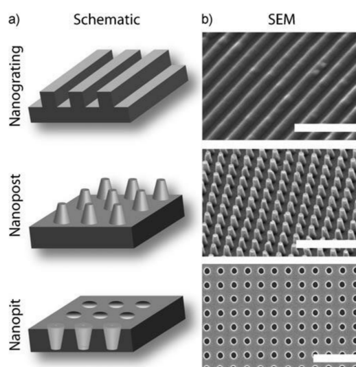
Figure 2. Schematic illustrations (a) and SEM images (b) of representative nanotopography geometries. Nanograting (scale bar = 5 \mu\text{m} ), nanopost (scale bar = 5 \mu\text{m} ), and nanopit array (scale bar = 1 \mu\text{m} ) [114].
