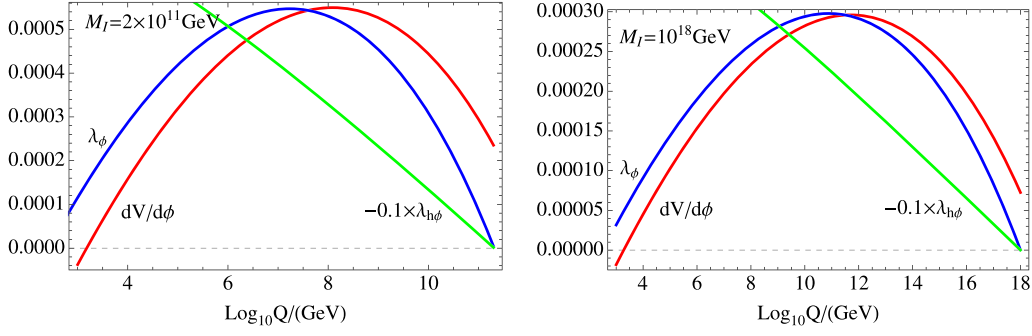
Fig. 1. Examples of running quartic coupling \lambda_\phi (blue), the minimization condition (12) (red), and \lambda_{H\phi} (green) (multiplied by -0.1 to fit in the plot) for the instability scale M_I = 2 \times 10^{11} GeV on the left and M_I = 10^{18} GeV on the right. Successful electroweak symmetry breaking occurs in both examples with the charge mixing parameter, x = 4/5 . (For interpretation of the references to color in this figure legend, the reader is referred to the web version of this article.)
