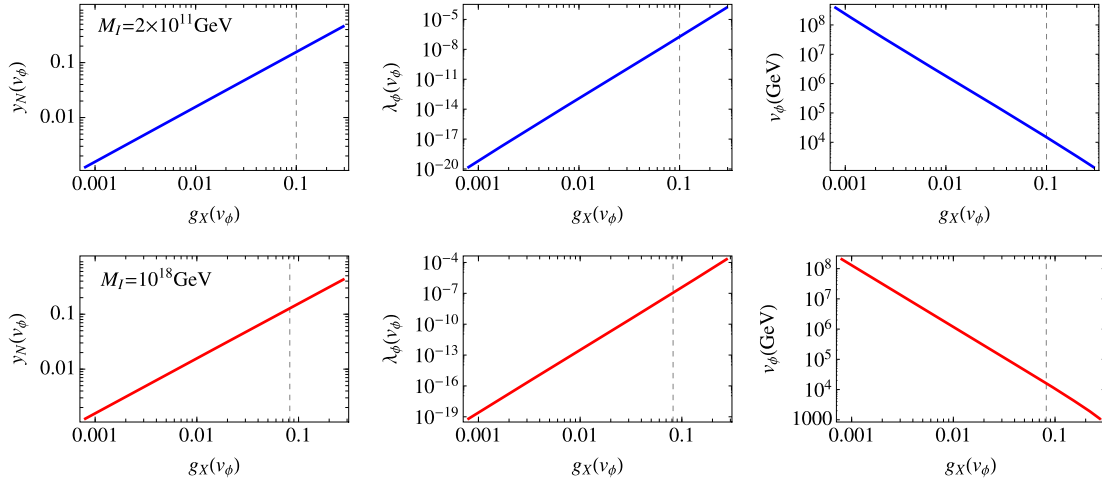
Fig. 2. The values of the gauge coupling g_X vs. the right-handed neutrino Yukawa coupling y_N (left), the quartic coupling \lambda_\phi (middle), and the U(1)_X breaking scale v_\phi (right) realizing successful electroweak symmetry breaking. We have chosen the charge mixing parameter to x = 4/5 , the Higgs mass at 126 GeV and the instability scale, M_I = 2 \times 10^{11} GeV and 10^{18} GeV, in the upper and lower panels, respectively. We get M_X > 3 TeV in the region left to the vertical dashed line.
