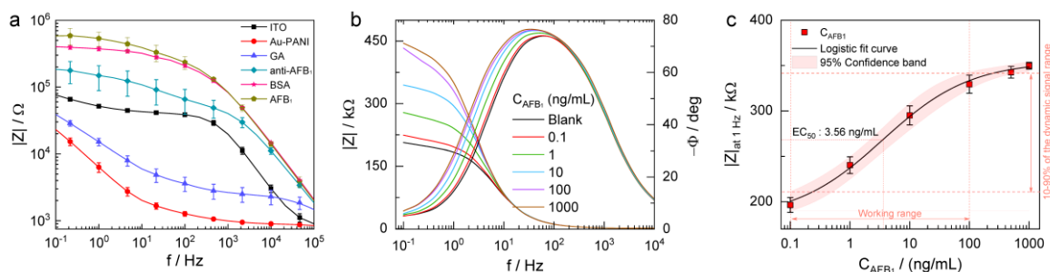
Figure 5. (a) Bode plots obtained after various steps of the surface modification process for (■) ITO; (●) Au-PANI; (▲) glutaraldehyde (GA); (◆) anti-AFB 1 ; (★) for BSA and (●) for AFB 1 (100 ng/mL) for developing the aflatoxin detection sensor. Data points indicate the mean \pm SD of four replicated impedance measurements; (b) Impedance magnitude measured from different concentration of aflatoxin B 1 ( C_{\text{AFB}_1} ) in phosphate buffer saline (PBS) measured from blank, 0.1 to 1000 ng/mL over the frequency range of 1 to 10^6 Hz; (c) Calibration curve with 95% confidence bands for AFB 1 sensor obtained at |Z|_{\text{at } 1 \text{ Hz}} for various C_{\text{AFB}_1} . Data points indicate the mean \pm SD of four replicated impedance measurements, and the fit curve represents the logistic four-parameter regression.
