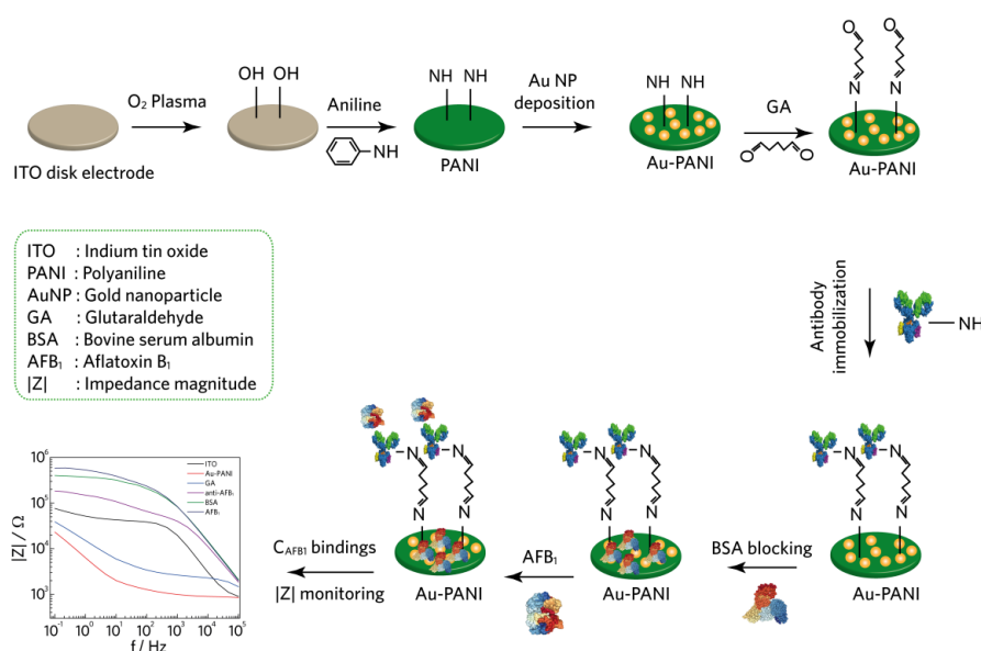
Figure 1. Schematic diagram showing a surface modification of Au–PANI-based disk electrodes for Aflatoxin B 1 binding with glutaraldehyde (GA) acting as a crosslinking agent to bind anti-AFB 1 to polyaniline (PANI) nanofibers.
