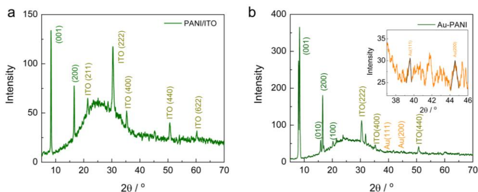
Figure 4. X-ray diffraction (XRD) patterns obtained for (a) PANI/ITO and (b) Au-PANI/ITO electrodes respectively; inset of Figure 4b shows the magnified view of the XRD peaks of Au nanoparticles in the range from 37–46 deg.
