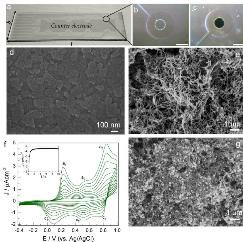
Figure 2. (a) Digital picture shows eight working indium tin oxide (ITO) disk electrodes along with large common counter electrode fabricated on glass substrates of dimension 7.5 \times 2.5 cm ( l \times b ), (b,c) optical images of bare ITO and Au-PANI coated ITO disk electrodes respectively. Scalebar is 500 \mu\text{m} . Scanning electron microscopy of (d) bare ITO; (e) PANI/ITO electrode; and (g) Au-PANI/ITO disk electrode surfaces respectively; (f) cyclic voltammogram obtained during potentiodynamic deposition of PANI on ITO electrodes at a sweep rate of 50 \text{ mV/s} . The highest current peaks belong to the 10th (the last) cycle. The chronoamperometric curve represents the Au deposition process for a duration of 10 s shown in the inset of Figure 2f.
