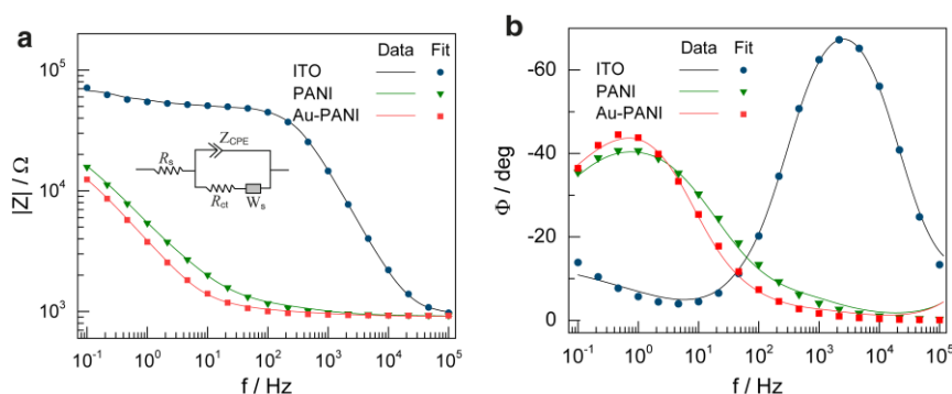
Figure 3. Bode plot shows (a) |Z| vs. f and (b) \Phi vs. f for bare ITO, PANI/ITO, and Au-PANI/ITO electrodes respectively. Inset of figure (a) shows the equivalent model circuit used to extrapolate the parameters through impedance fitting analysis.
