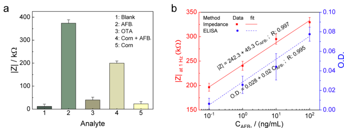
Figure 6. (a) Selectivity of the developed sensor demonstrated by impedance measurements with various types of the analyte to examine the cross-reactivity of the AFB 1 sensor; (b) impedance change and optical density (O.D.) obtained by ELISA versus AFB 1 concentrations (0.1 to 100 ng/mL).
