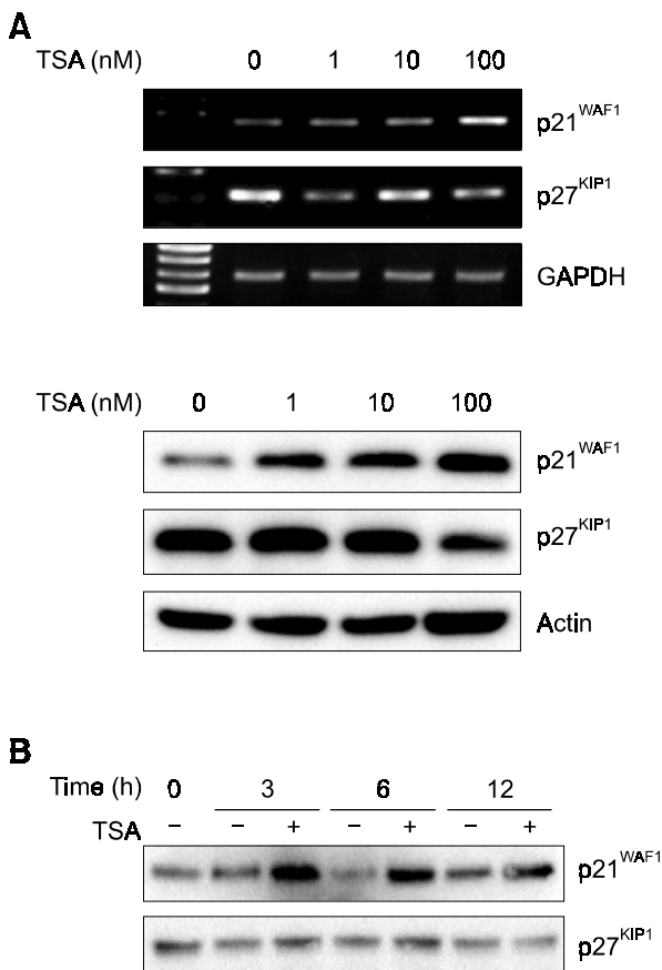
Figure 3. TSA causes upregulation of p21 WAF1 in osteoclasts. (A) Osteoclast cultures, prepared as described above, were treated with TSA for 12 h. The expression levels of transcripts (upper panel) and proteins (lower panel) of p21 WAF1 and p27 KIP1 were analyzed by semi-quantitative RT-PCR and western blotting, respectively. GAPDH and actin served as loading controls for the RT-PCR and western blots, respectively. (B) Cultures were treated with 100 nM TSA for the indicated periods and p21 WAF1 and p27 KIP1 proteins were analyzed by western blotting. Similar results were obtained from three independent experiments. Representative results are shown.
