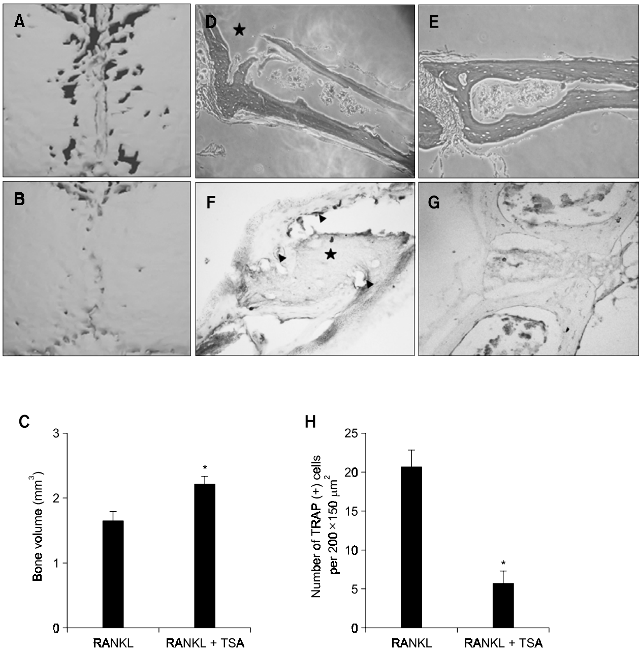
Figure 5. TSA inhibits RANKL-directed bone destruction in vivo . Collagen sponges soaked with RANKL or RANKL plus TSA were placed on the center of sagittal suture on the calvaria. After 2 days of treatment, calvariae were collected and analyzed by \mu CT (A-C) and histology with H-E staining (D, E) and TRAP staining (F-H). Reconstructed \mu CT views of calvariae treated with RANKL and RANKL plus TSA are shown in (A) and (B), respectively. Bone volumes were measured from four animals per group by \mu CT in the regions shown in A and B (C). H-E staining views of RANKL (D) and RANKL plus TSA (E). TRAP staining views of RANKL (F) and RANKL plus TSA (G). Number of TRAP(+) cells attached on bone surface were counted in 4 mm-wide area along the sagittal suture (H). The stars in D and F indicate disruption of diploë, and the arrow heads in F indicate TRAP(+) osteoclasts which were counted. Data are averages \pm SDs ( n = 4 ). *Statistically significant (Student's t -test, P < 0.05 ).
