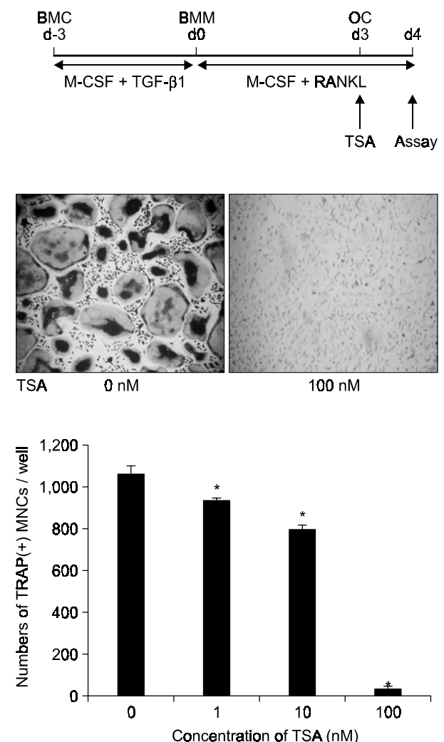
Figure 1. TSA treatment of osteoclasts reduces the number of TRAP-positive MNCs. BMMs were induced to differentiate to osteoclasts (OCs) by exposure to RANKL and M-CSF for 3 days. The osteoclasts were treated with TSA for 24 h in the presence of RANKL and M-CSF, followed by TRAP staining. TRAP-positive cells containing three or more nuclei were counted under the microscope. Representative images are presented. Data are averages \pm SDs ( n = 3 ). *Statistically significant (Student's t -test, P < 0.05 ).
