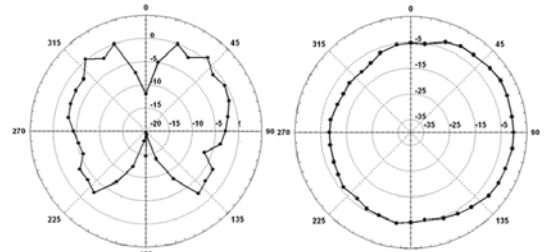
(c) E-평면(off 상태) xz 평면( \phi=0^\circ ) (c) E-plane(off state) xz plane( \phi=0^\circ )
