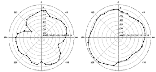
(a) E-평면(on 상태) yz 평면( \phi=90^\circ ) (a) E-plane(on state) yz plane( \phi=90^\circ )
