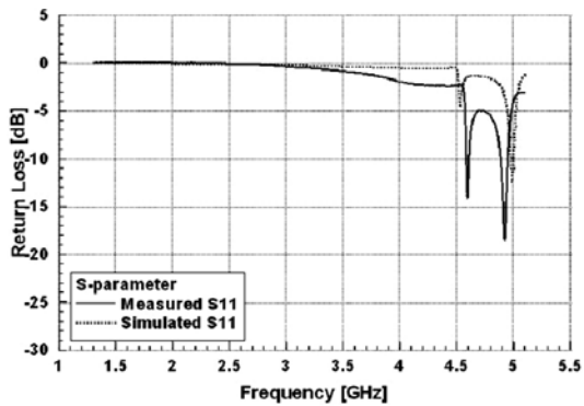
(b) Off 상태 (b) Off state
