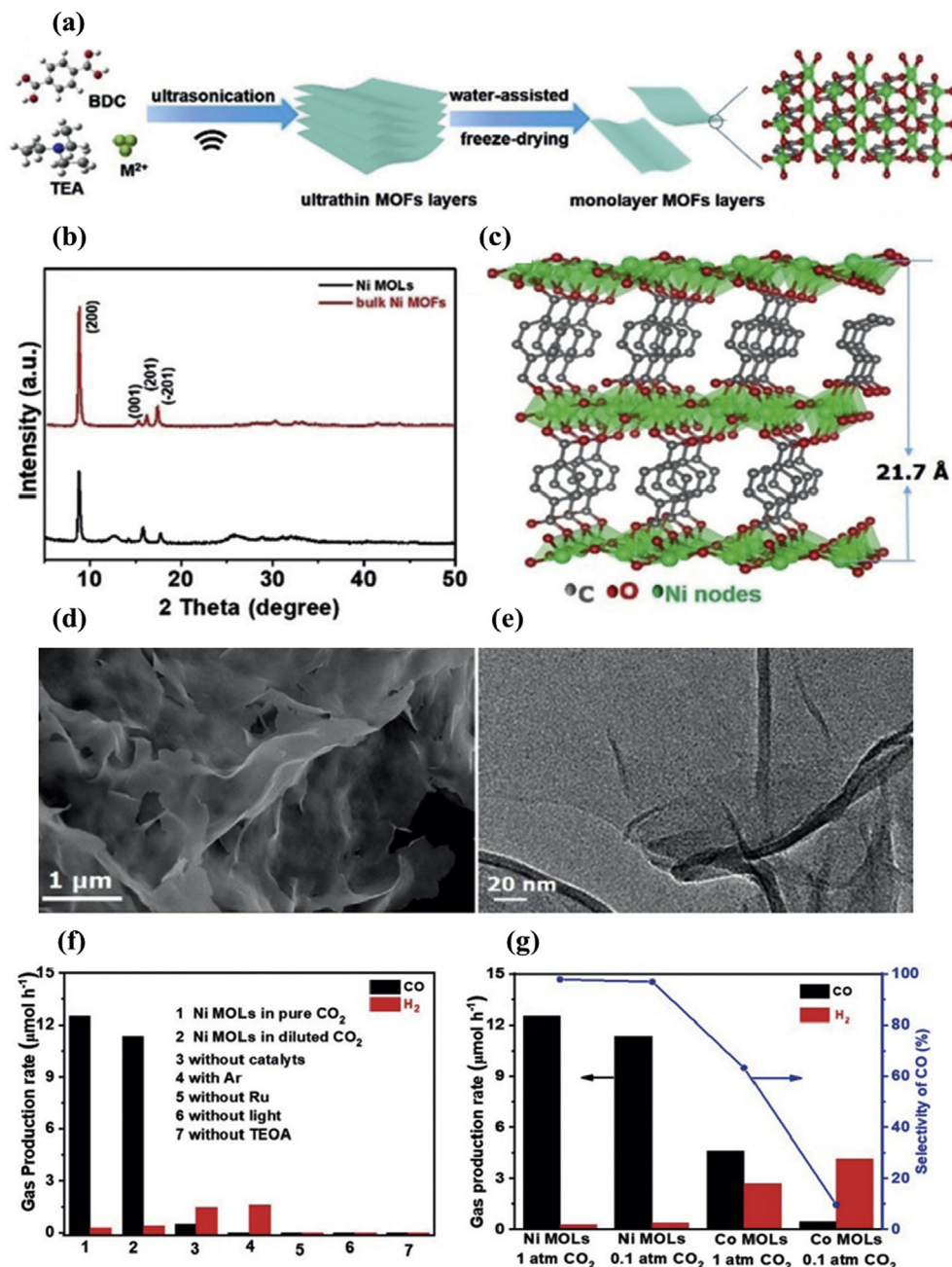
Fig. 13. (a) A schematic illustration of the generation of Ni MOFs, (b) XRD pattern, (c) atomic arrangement, (d) SEM image, (e) TEM image of Ni MOFs, (f) CO 2 photoreduction performance under various reaction conditions, and (g) CO 2 photoreduction performance over Ni MOFs and Co MOFs in pure and diluted (10%) CO 2 . Reproduced with permission [214]; Copyright 2018, Wiley-VCH.
