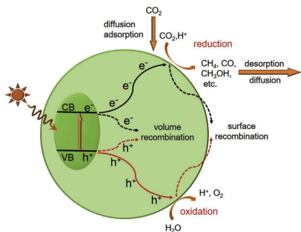
Fig. 2. An illustration of photocatalysts for CO 2 reduction reaction. Reproduced with permission [98]; copyright 2018, WILEY-VCH.
