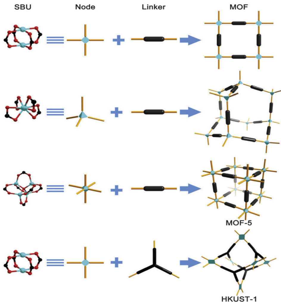
Fig. 8. A graphical illustration of the construction of some MOFs from SBU and rigid linkers. Reproduced with permission [155]; Copyright 2014 Chemical Society Reviews.
