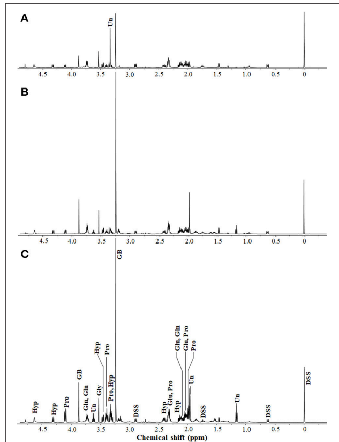
FIGURE 1 | 1 H-NMR spectra of extracts from H. halophilus cells grown in marine broth containing 0.4 (A), 1.0 (B), and 2.5 M (C) NaCl. Sodium 2,2-dimethyl-2-silapentane-5-sulfonate (DSS; 5 mM) was used as the internal standard. Intracellular organic compounds from the 1 H-NMR spectra were identified with the Chenomx NMR suite. 1 H-NMR peaks corresponding to glutamate (Glu), glutamine (Gln), glycine betaine (GB), proline (Pro), glycine (Gly), and trans-4-hydroxy-L-proline (Hyp) are indicated. Unidentified intracellular organic compounds (Un) that responded to changes in NaCl concentrations are also shown.
