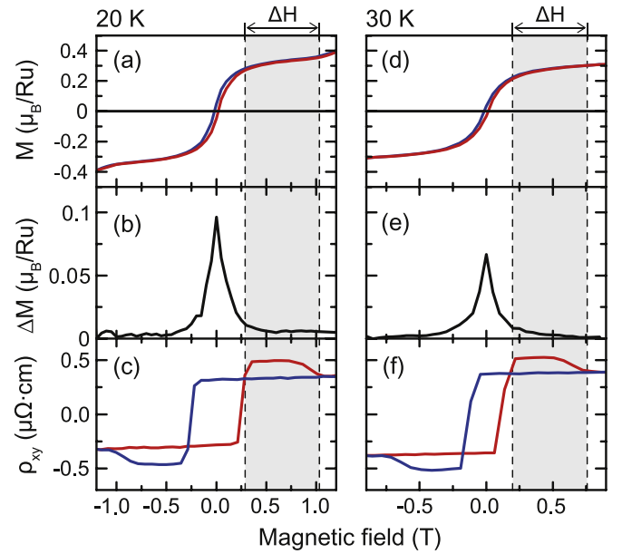
Fig. 3. (a) Normalized M - H curve of 4 u.c. SRO film measured with out-of-plane field direction at 20 K. Diamagnetic signal from the STO substrate has been subtracted. Red (blue) line represents the positive (negative) sweep direction of the applied magnetic field. Clear hysteresis is observed. (b) The difference between the two magnetizations measured with positive and negative sweep directions (difference between the two curves in (a)). (c) Hall resistivity \rho_{xy} of the 4 u.c. SRO film measured at 20 K. (d), (e) and (f) Corresponding data set measured at 30 K. The dashed lines indicate the fields at which the magnetization nearly saturates ( \Delta M = 0 ) and the hump disappears, respectively. (For interpretation of the references to colour in this figure legend, the reader is referred to the Web version of this article.)
