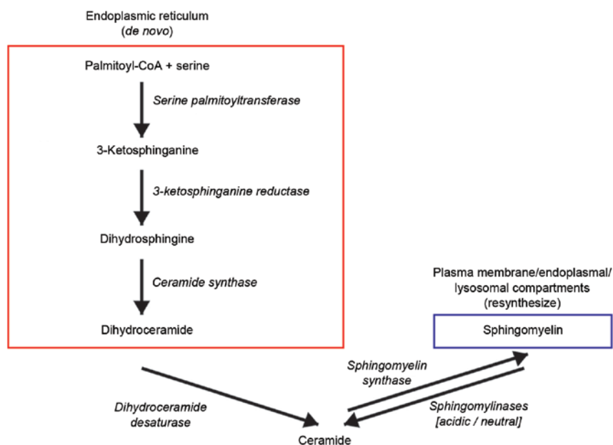
Figure 1. Biochemical pathway of ceramide generation and metabolism. Enzymes are shown in italics. Ceramide is derived from two main pathways operating in different cellular compartments: De novo synthesis from serine and palmitoyl CoA; and hydrolysis of membrane-derived sphingomyelin.
