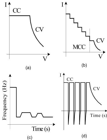
FIGURE 4. Traditional and advanced charging techniques.
