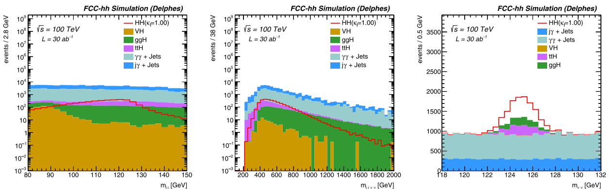
Fig. 126. Left: Di-jet system invariant mass spectrum before applying the di-jet invariant mass selection. Di-Higgs (centre) and di-photon (right) candidates invariant mass spectra after applying all selection criteria.
