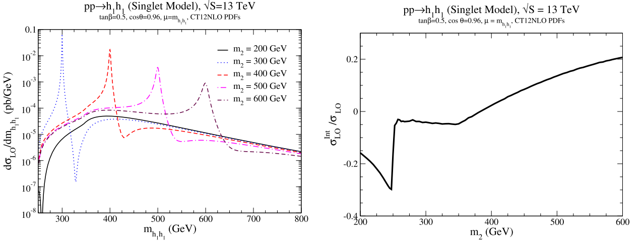
Fig. 31. Left: Invariant mass distributions of di-Higgs final state in the Z_2 symmetric singlet model for various singlet masses. Right: Fractional contribution of the interference of h_2 s-channel contribution with h_1 s-channel and box diagram contributions Ref. [195].
