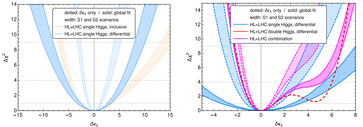
Fig. 27. HL-LHC at 13 TeV and 3 ab -1 . Left: Single Higgs with only inclusive measurements (orange) and including differential information (blue) with only \kappa_\lambda (pale colour) or marginalising over the nine EFT coefficients (strong colour). Right: Constraints from differential single Higgs (blue), differential double Higgs (dashed red) and their combination (pink). (For interpretation of the references to colour in this figure legend, the reader is referred to the web version of this article.)
