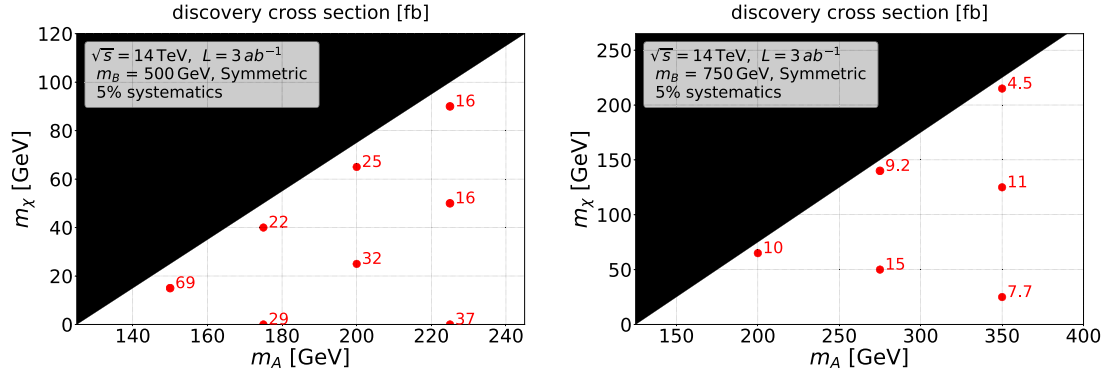
Fig. 53. Cross sections (in fb) for the 4b2\chi final state required for a discovery at the HL-LHC in the m_A - m_\chi plane for the symmetric model, with m_B = 500\text{ GeV} (left panel) and m_B = 750\text{ GeV} (right panel) [358].
