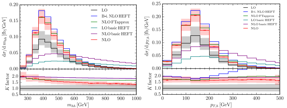
Fig. 5. Higgs pair invariant mass and transverse-momentum distributions for a center-of-mass energy of 14 TeV in various approximations. The full NLO results are shown in red. The red bands show the renormalization and factorization scale dependence obtained from a 7-point scale variation around the central scales \mu_R = \mu_F = m_{HH}/2 [18]. (For interpretation of the references to colour in this figure legend, the reader is referred to the web version of this article.)
