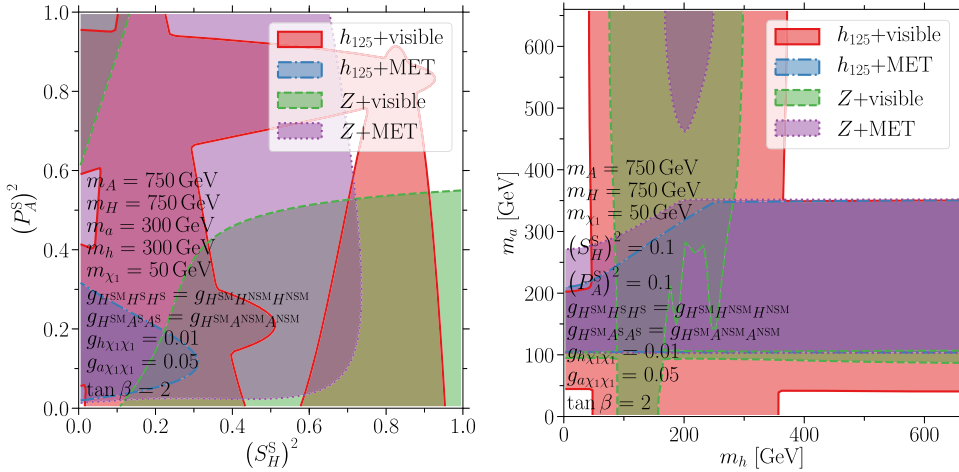
Fig. 38. Regions of 2HDM + S parameter space within the future reach of the different Higgs cascade search modes as indicated in the legend at the LHC with \mathcal{L} = 3000\text{fb}^{-1} of data. The left panel shows the accessible regions in the plane of the parent Higgs bosons (S_H^S)^2 vs (P_A^S)^2 . The right panel shows the reach in the plane of the masses of the daughter Higgs bosons produced in the Higgs cascades, m_h vs m_a . The remaining parameters are fixed to the values indicated in the labels [273].
