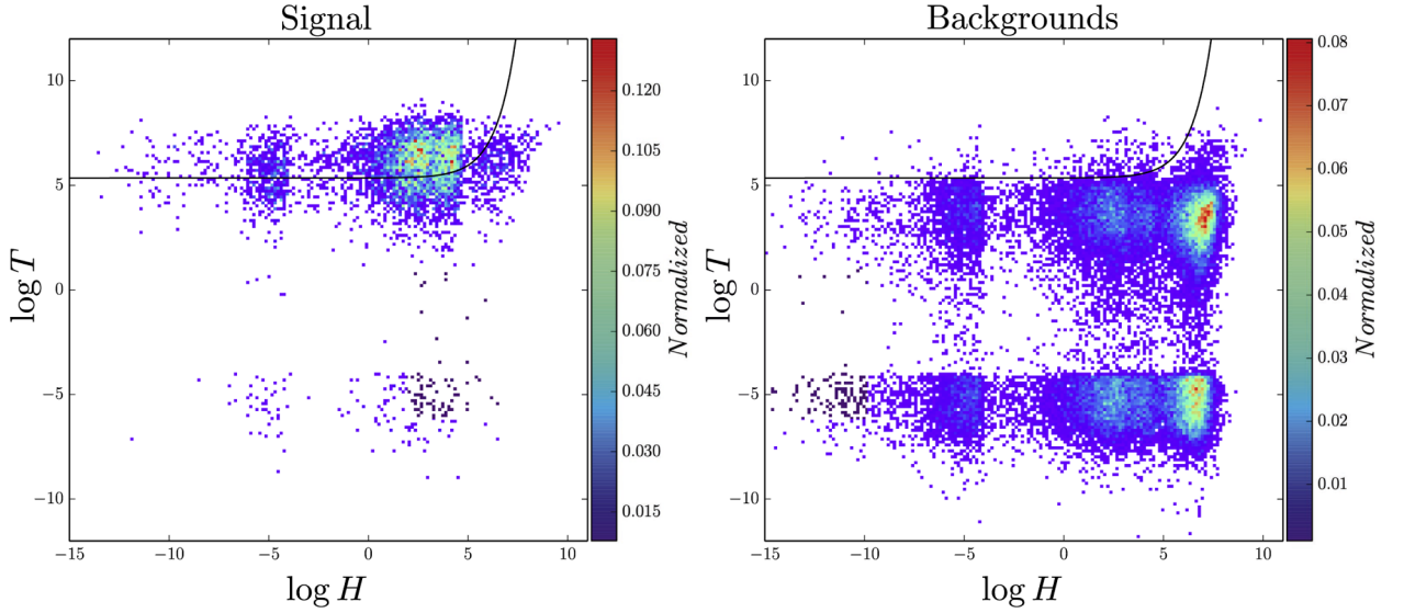
Fig. 76. Distribution of (\log H, \log T) for simulated signal ( HH ) and backgrounds ( t\bar{t} , t\bar{t}H , t\bar{t}V , \ell\bar{\ell}b\bar{b} , b\bar{b}\tau^+\tau^- and others) events after loose selection requirements as defined in Ref. [457].
