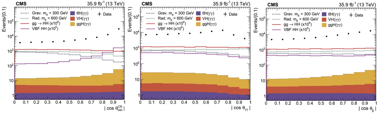
Fig. 69. Distributions of the three helicity angles for data (dots), \gamma +jets background, different signal hypotheses and three single Higgs boson samples ( t\bar{t}H , VH , and ggH ) after the selections on photons and jets [442] have been applied.
