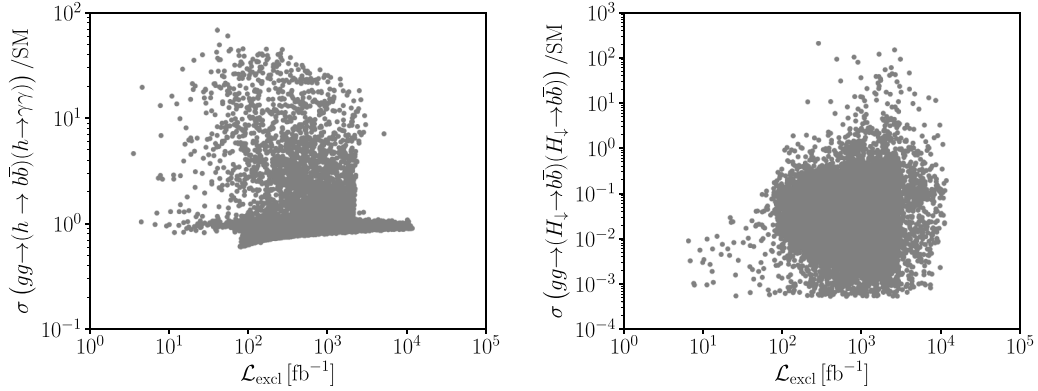
Fig. 37. Higgs pair production cross sections normalised to the SM value for SM-like Higgs pairs decaying into b\bar{b}\gamma\gamma (left) and light-non-SM-like Higgs pairs decaying into b\bar{b}b\bar{b} (right) as a function of the exclusion luminosity, for the C2HDM T1 scenarios passing our applied constraints [265,266].
