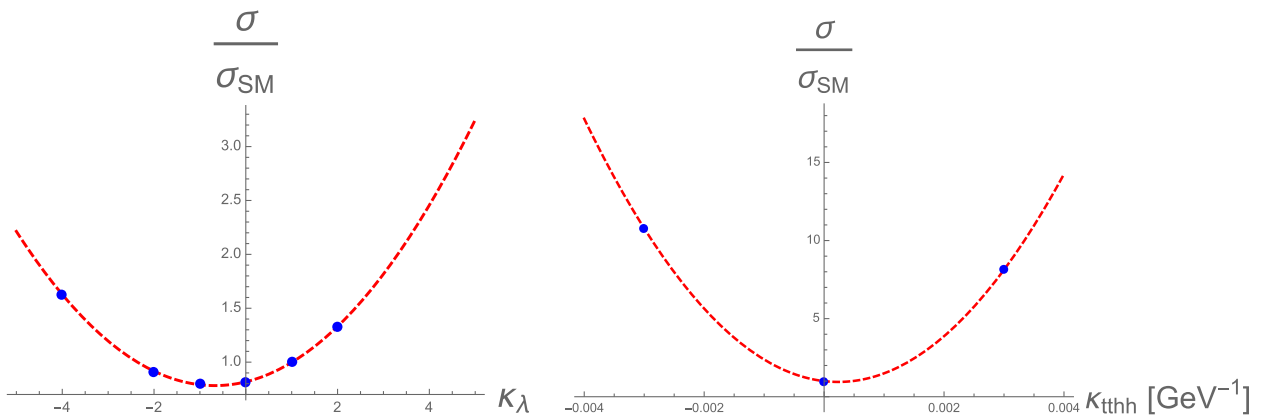
Fig. 137. \sigma/\sigma_{\text{SM}} as a function of \kappa_\lambda (left) and \kappa_{t\bar{t}HH} [GeV -1 ] (right), where \kappa_{t\bar{t}HH} = -m_t c_H/v^2 .
