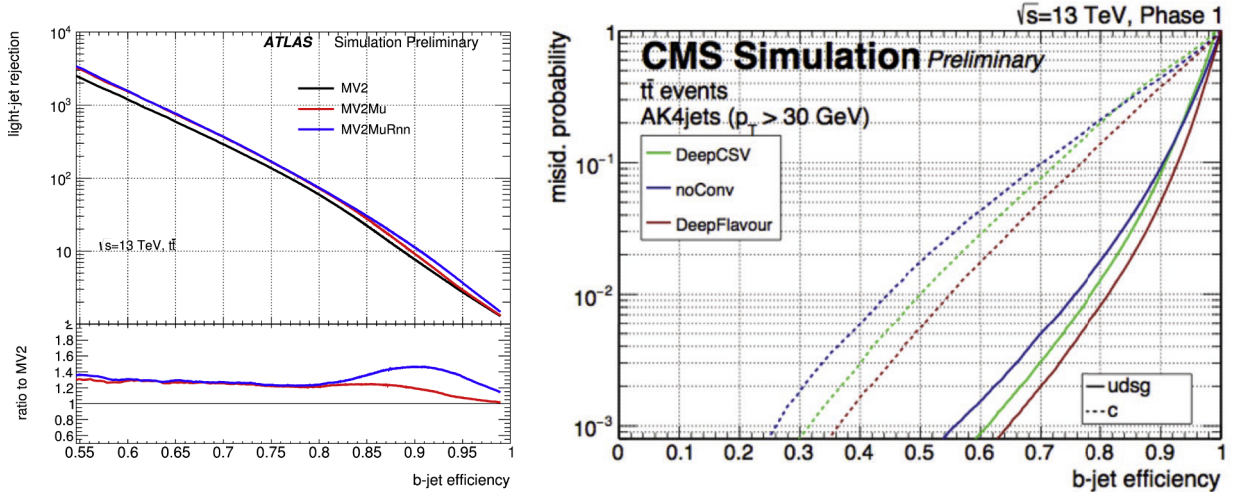
Fig. 55. Light-flavour rejection as a function of b -jet efficiency for DNN-based algorithm developed by ATLAS: MV2, MV2Mu and MV2MuRNN. The performance are evaluated for jets with p_T > 20\text{ GeV} (left) [387]. Comparison between the DeepCSV and DeepFlavour algorithms developed by CMS (right). The plot shows the b -tagging efficiency versus the mis-tag rate from light-jets (continuous line) and c -jets (dashed line) evaluated for jets with p_T > 30\text{ GeV} . [389].
