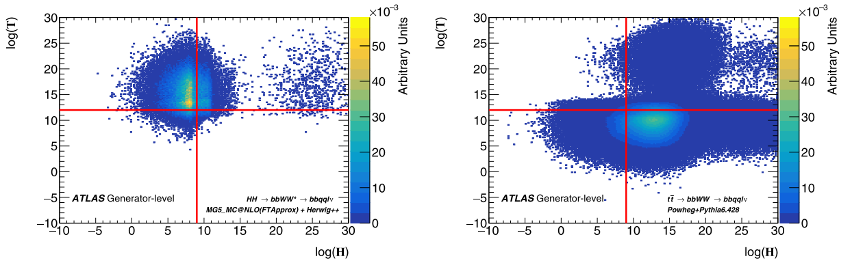
Fig. 78. Distribution of Higgsness and Topness ( \log(H) , \log(T) ) for simulated signal HH \rightarrow b\bar{b}WW^* \rightarrow b\bar{b}qq\ell\nu and background t\bar{t} \rightarrow b\bar{b}WW^* \rightarrow b\bar{b}qq\ell\nu events without selection requirements. The signal has been simulated with MG5_AMC@NLO using the FTApprox approximation and with a HERWIG++ parton-shower simulation, while the background sample is generated with POWHEG and PYTHIA 6.428. The distributions are normalised to unit area. Red lines are drawn to give a visible reference for a possible separation between signal and background [501].
