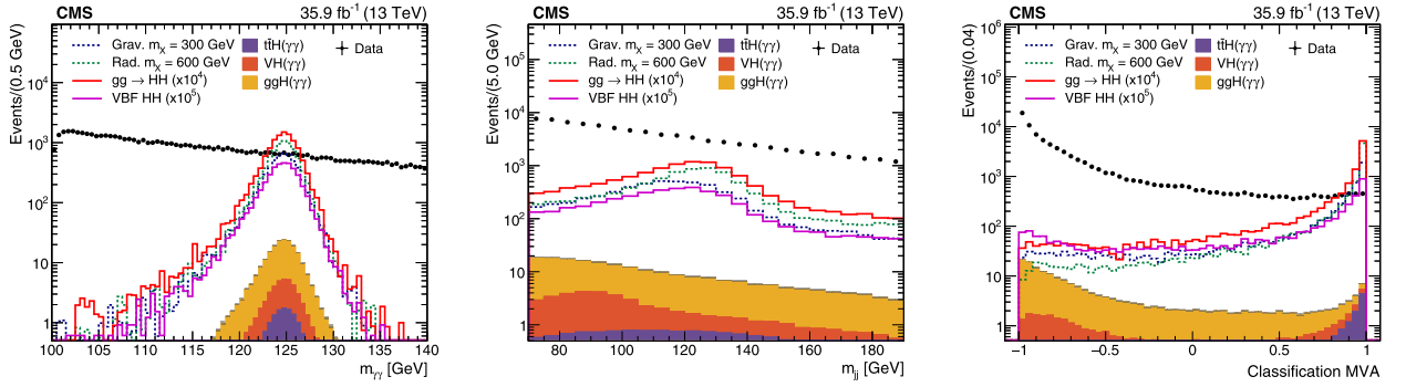
Fig. 85. Higgs candidate m_{\gamma\gamma} (left) and m_{jj} (middle) distributions, as well as the BDT classifier score (right) in the CMS HH \rightarrow b\bar{b}\gamma\gamma analysis after kinematic selection criteria are applied. The contribution of the VBF HH process is shown in pink, normalised to 10^5 times its cross section [442].
