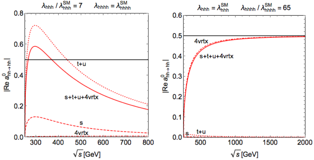
Fig. 20. Dependence of the J = 0 partial wave a^0 on the centre of mass energy \sqrt{s} for modified trilinear Higgs self-coupling (left) and modified quartic Higgs self-coupling (right). The plots are taken from Ref. [151].
