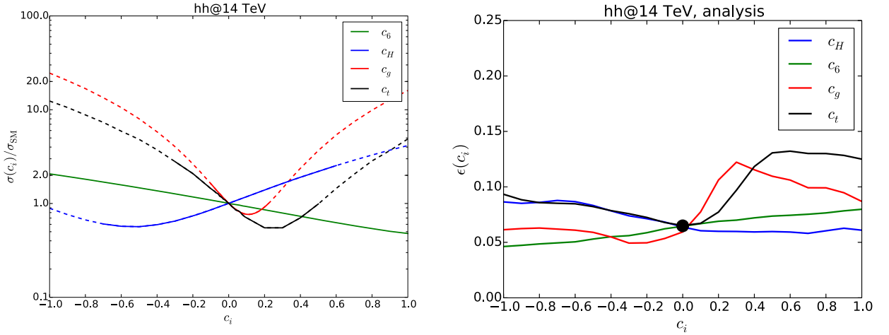
Fig. 23. Left: Relative change in the HH cross section in dependence on individual operators. The dashed parts of the curves are excluded at 95% CL from Higgs boson data. Right: Corresponding efficiency of the analysis. See text for details.
