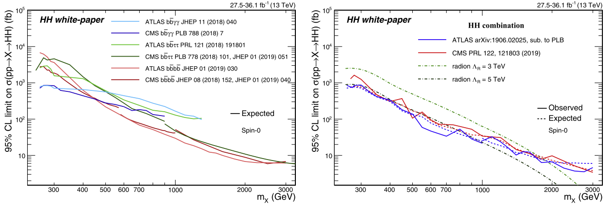
Fig. 99. Top: expected 95% CL upper limits on the resonant production cross section of a narrow, spin-0 resonance (S or X) decaying into a pair of Higgs bosons for the most sensitive channels: b\bar{b}b\bar{b} , b\bar{b}\tau^+\tau^- and b\bar{b}\gamma\gamma . Bottom: expected and observed 95% CL combined exclusion limits on the resonant spin-0 HH production. A theory prediction from bulk radion model is overlaid [531,532].
