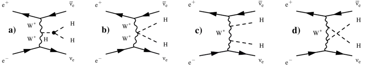
Fig. 111. Diagrams contributing to e^+e^- \rightarrow \nu\bar{\nu}HH .
