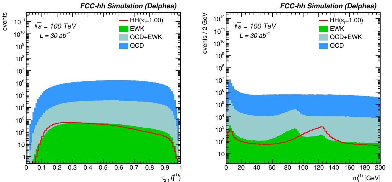
Fig. 130. 2-to-1 ( \tau_{2,1} ) subjettness ratio (left) and soft-drop mass (left) spectra of the leading Higgs large-radius jet candidate.
