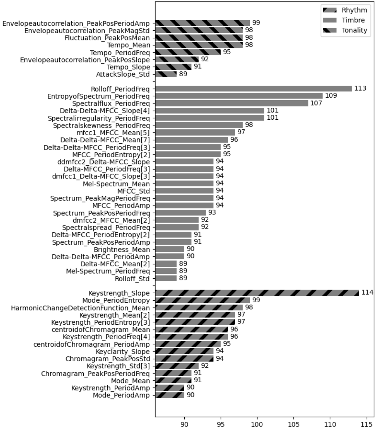
FIGURE 2. Top 50 frequently selected features and the number of times selected across the entire experiment (Features in Rhythm, Timber, Tonality field given by MIRtoolbox represented in different style).
