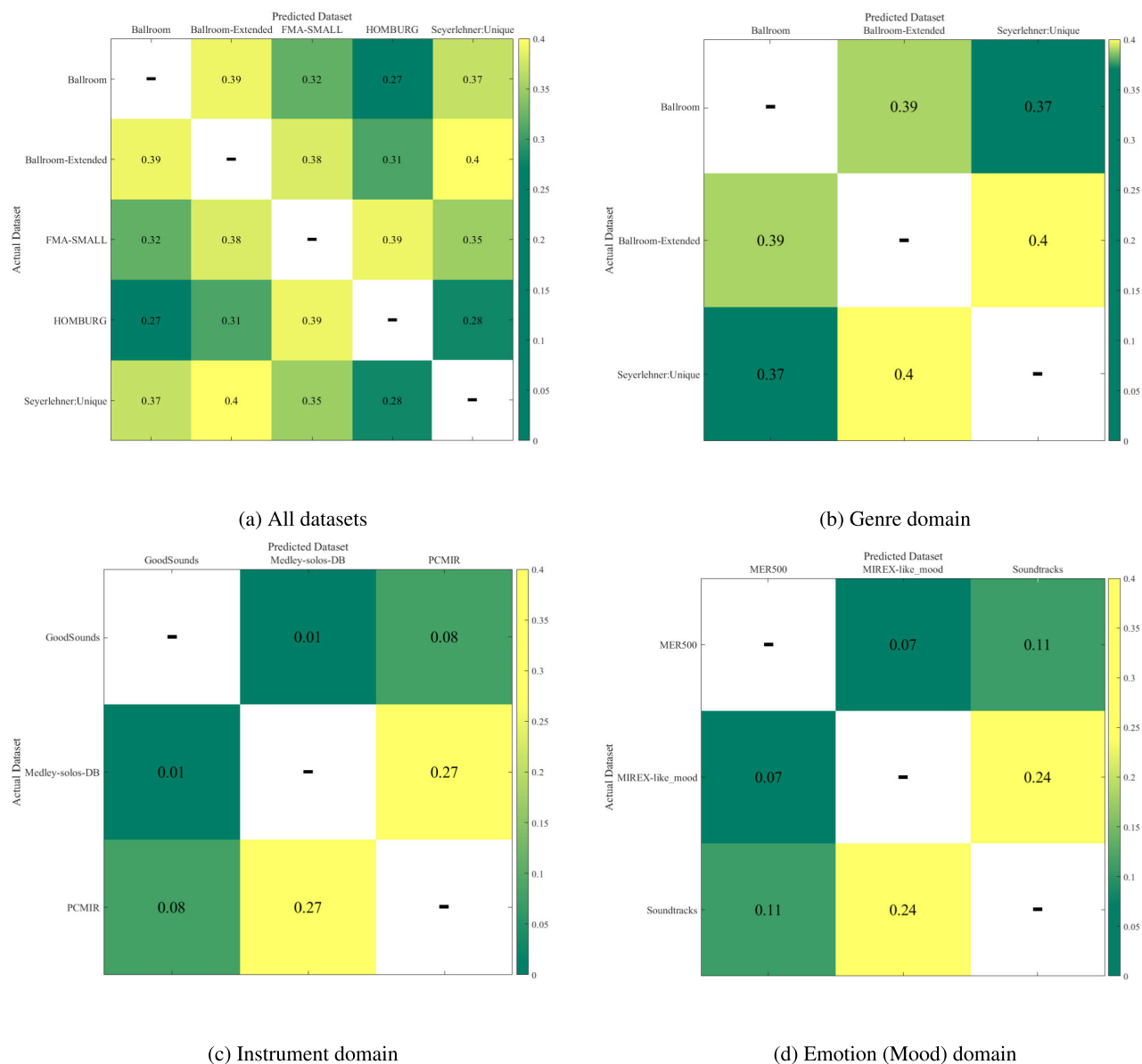
FIGURE 3. Dataset pairs with the highest correlation coefficient values.
