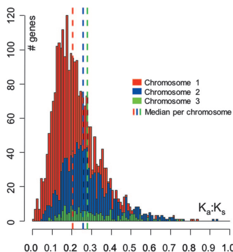
Fig. 3. The ratio of nonsynonymous vs. synonymous nucleotide substitutions ( K_a/K_s ) between orthologous pairs in LB400 and Bcc strain 383, plotted conjointly for the three chromosomes. There is a significant trend toward more spread ratios (flattening of the distribution) going from the large chromosome to the smaller ones. Although no positive selection could be evidenced overall for any pair of genes compared (i.e., K_a > K_s ), this trend can be interpreted as a progressive relaxation of the selection pressure for amino acid substitution (pressure Chr1 > Chr2 > MP) (cf. Fig. 5).
