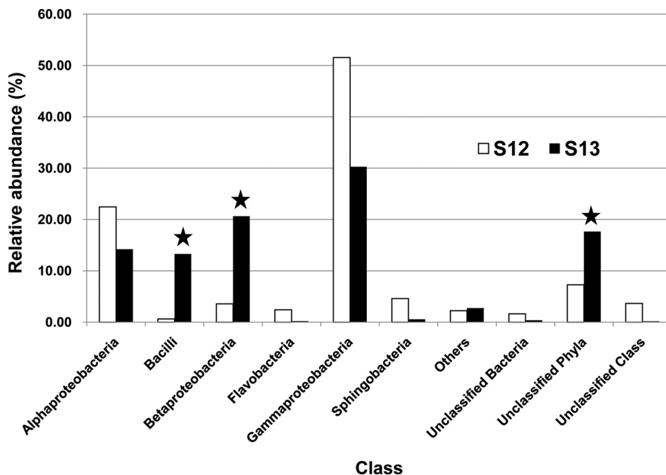
FIG. 1. Relative abundances of [12C]DNA (S12) and [13C]DNA (S13) in microbial community members. RDP Classifier was used at the class level with a 50% bootstrap threshold (4). Solid stars indicate the class members that exhibited significant enrichment in S13 compared to S12.
