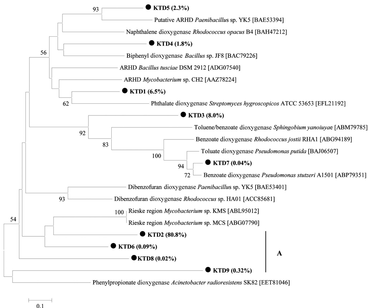
FIG. 2. Neighbor-joining phylogenetic tree (1,000 bootstraps) based on approximately 100-amino-acid sequences of ARHD genes. The Korean tidal flat dioxygenase (KTD) sequences are marked by dark circles. The number in the parentheses after each KTD sequence indicates the percentage of sequences in that cluster.
