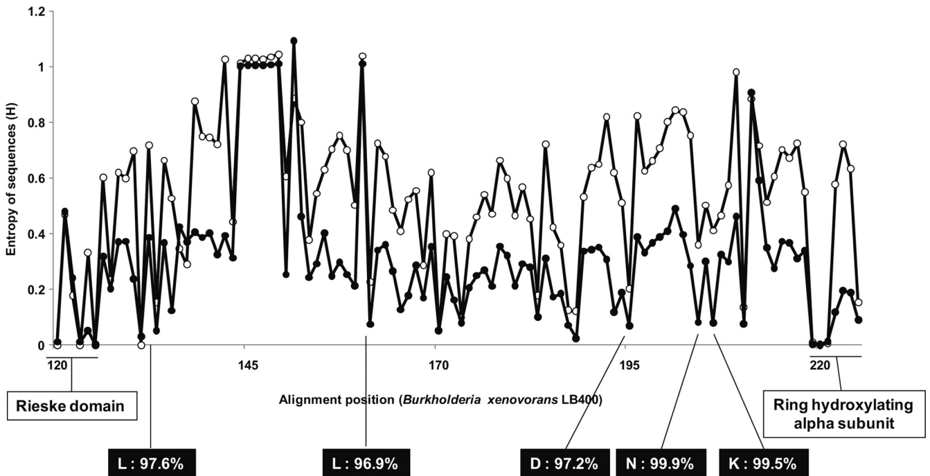
FIG. 3. Shannon entropy ( H' ) at each alignment position and conserved residues among the obtained and reference ARHD sequences. Open circles indicate the entropy of reference sequences, and solid circles indicate the entropy of the SIP-enriched (obtained) sequences. Known domains, amino acids, and their percentages of the total obtained sequences are shown in boxes.
