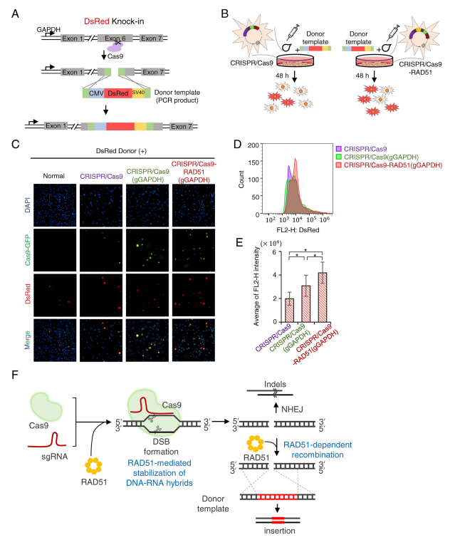
Fig. 4. RAD51 promotes the knock-in efficiency of CRISPR/Cas9. (A) Knock-in process of DsRed cassette. sgRNA targeting the terminal region of exon 6 of the GADPH gene cuts that locus, allowing genomic integration of the DsRed cassette through HDR. (B) Cartoon for DsRed-expressing cells by CRISPR/Cas9-mediated knock-in system. (C) Representative images showing DsRed expression in CRISPR/Cas9 system (GFP) through the knock-in process. Due to the exogenous promoter of the DsRed cassette, the expression of DsRed was shown in normal condition. (D) Histogram describes the cell number according to the amount of DsRed intensity in each condition. (E) Quantitative analysis of FL2-H implying DsRed fluorescence measured in (D). Error bars indicate the mean \pm SD ( n = 3 ). Statistical significance, * P < 0.05 , ** P < 0.01 , *** P < 0.001 . (F) Proposed working mechanism of RAD51-mediated CRISPR/Cas9 system.
