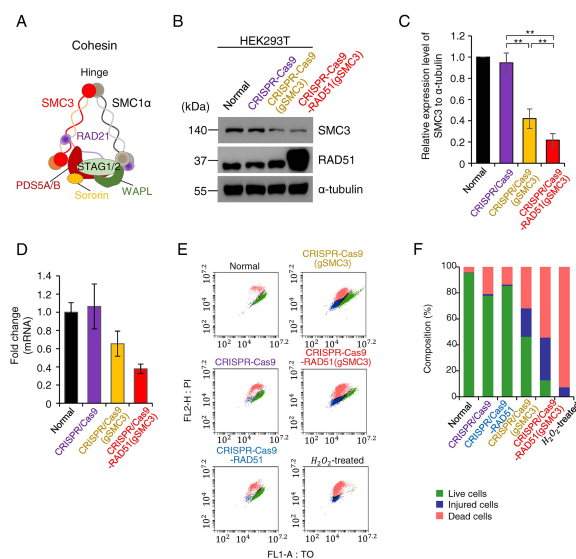
Fig. 3. Impact of RAD51 on SMC3-targeting CRISPR/Cas9 knock-out process. (A) Compositional structure of mitotic cohesin; SMC3 is indicated in bright red. (B) Expression analysis of SMC3 targeted by CRISPR/Cas9. Protein levels were detected through immunoblot assay. (C) Quantification of SMC3 protein levels in (B). Relative SMC3 protein level to \alpha -tubulin was normalized to the sample of non-transfected mock. Error bars indicate the mean \pm SD ( n = 3 ). Statistical significance, * P < 0.05 , ** P < 0.01 , *** P < 0.001 . (D) qPCR analysis of SMC3 gene in each CRISPR/Cas9 plasmid. The fold-change value was normalized to the numerical value of the non-transfected mock. Error bars indicate the mean \pm SD ( n = 3 ). (E) Cell viability assay to observe the effect of SMC3 depletion. Each cell sorting (live, injured, and dead cells) was based on the distributions of mock and H_2O_2 -treated samples. (F) The proportion of each cell composition in indicated conditions was quantified.
