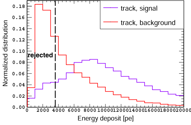
FIG. 25. The total energy deposit of the first object in time in the track case. Neutron-induced track deposits larger energy.
