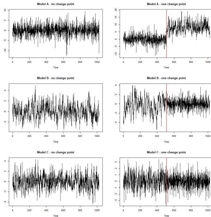
Figure 3: Randomly selected time series from Model A (top), Model B (middle), and Model C (bottom), under T = 1024 , and three time series on the right panels contain structural changes at t_0 = 512 , marked with red vertical lines.
