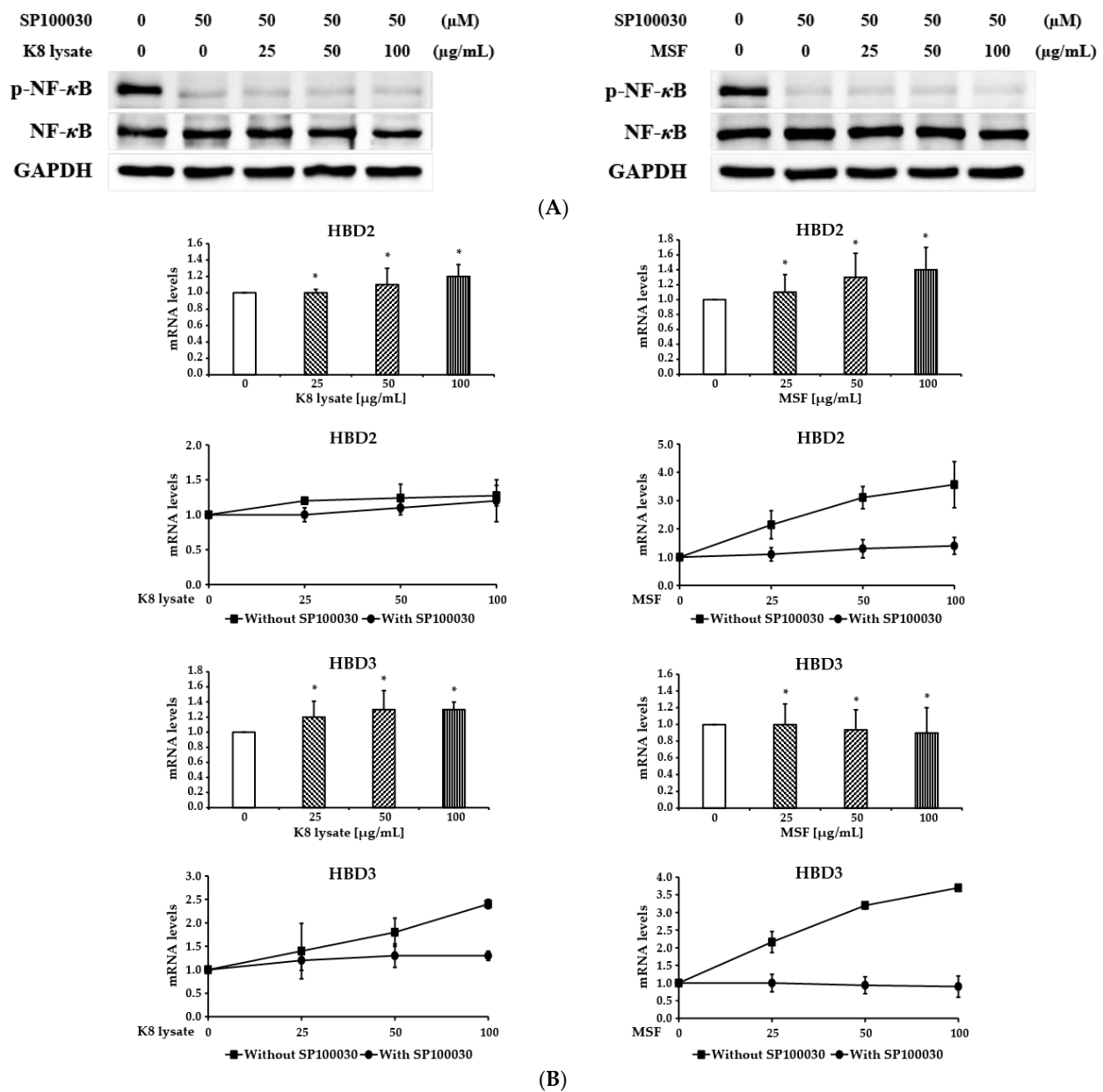
Figure 4. MSF increased the expression of HBD3 through the NF-κB signaling pathway. HaCaT cells were pre-treated with SP100030 (50 μM) for 3 h and then treated with 25 to 100 μg/mL of MSF or K8 lysate for 1 h. (A) The expression of NF-κB and the phosphorylated form of NF-κB were detected by Western blot. (B) The expressions of HBD2, and HBD3 were checked by qRT-PCR in a NF-κB-inhibited condition. Results are representative of three biological replicates. * p < 0.05.
