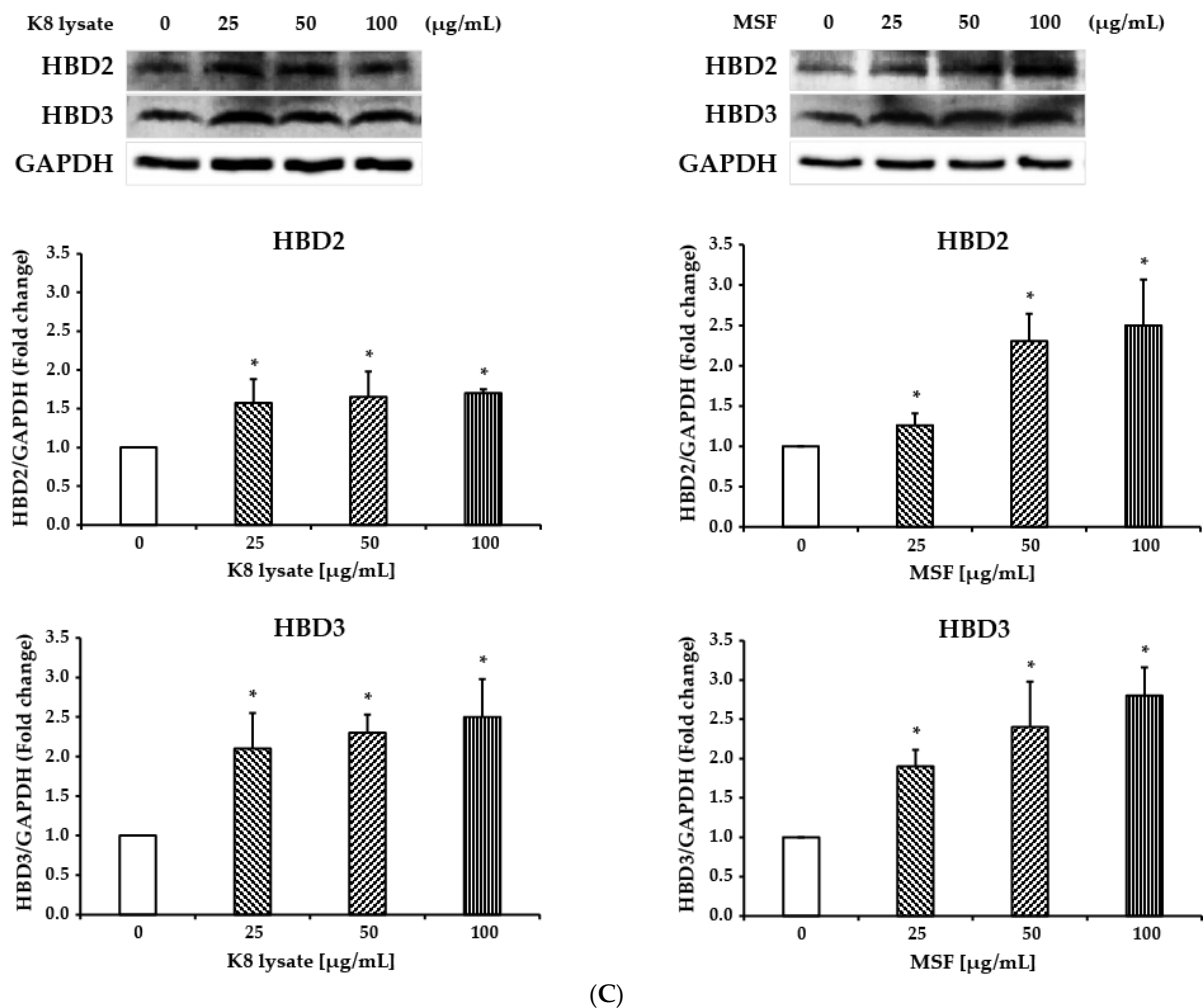
Figure 1. MSF induced the expression of the human antimicrobial peptide human \beta -defensin-2 (HBD2) and \beta -defensin-3 (HBD3). (A,B) qRT-PCR analysis of HBD1, HBD2, and HBD3 mRNA levels in HaCaT after treatment with MSF or K8 lysate. (C) The protein expression of HBD2 and HBD3 was increased by MSF treatment in HaCaT cells for 1 h and Western blot quantification was checked by ImageJ. Values are mean \pm SD from three independent experiments. * p < 0.05 , ** p < 0.01 .
