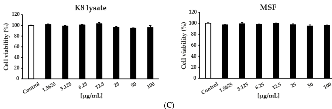
Figure 2. MSF induced the NF- \kappa B and p38 protein levels in HaCaT cells. After 20 h of starvation, HaCaT cells were treated with 25–100 \mu g/mL of MSF or K8 lysate for 1 h. (A,B) Western blot analysis of PI3K, AKT, NF- \kappa B, JNK, ERK1/2, and p38 protein levels and Western blot quantification (the white bar is the phosphorylated form, and the black bar is the unphosphorylated form). (C) Viability of HaCaT cells after treatment with 1.5625–100 \mu g/mL of MSF or K8 lysate. Values are mean \pm SD from three independent experiments. * p < 0.05 , ** p < 0.01 .
