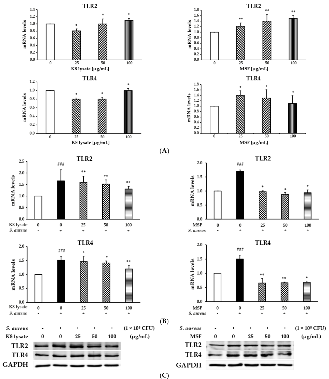
Figure 6. MSF treatment inhibited the expression of TLR2 in HaCaT and THP1 cells. (A) qRT-PCR analysis of TLR2 and TLR4 in HaCaT cells treated with 25–100 μg/mL of MSF or K8 lysate. (B) qRT-PCR analysis of TLR2 and TLR4 in THP1 cells stimulated by S. aureus treated with MSF or K8 lysate. (C) Western blot analysis. Data represent mean ± SD from three independent experiments. ### p < 0.001 vs. control. * p < 0.05 , ** p < 0.01 vs. model.
