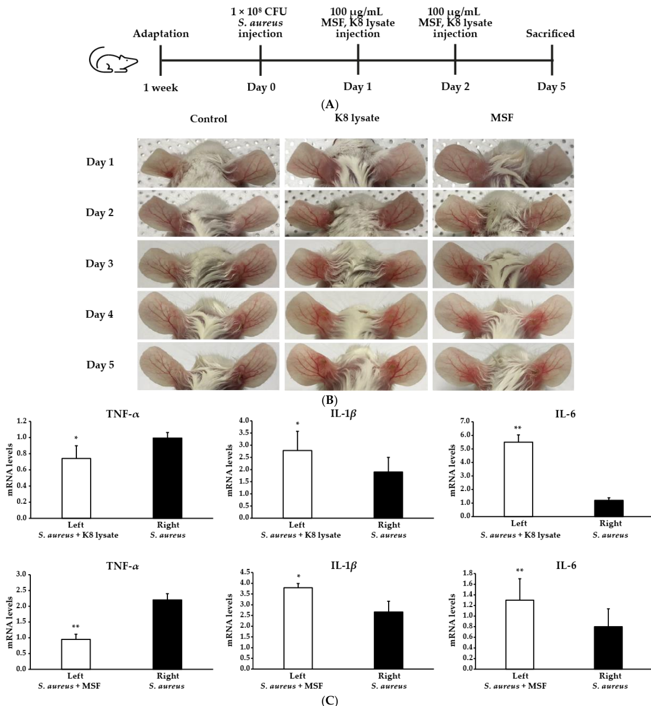
Figure 7. MSF reduced inflammation in an S. aureus -injected ears of a mouse model. Live S. aureus ( 1 \times 10^8 CFU) were inoculated into the ear of mice together with or without MSF or K8 lysate (100 \mu\text{g/mL} ). (A) Experimental scheme for in vivo studies. (B) Ears with an inflammatory phenotype. (C) The mRNA of TNF- \alpha , IL-1 \beta , and IL-6 expression levels were measured from the ears tissues using qRT-PCR. * p < 0.05 , ** p < 0.01 vs. right mouse ear.
