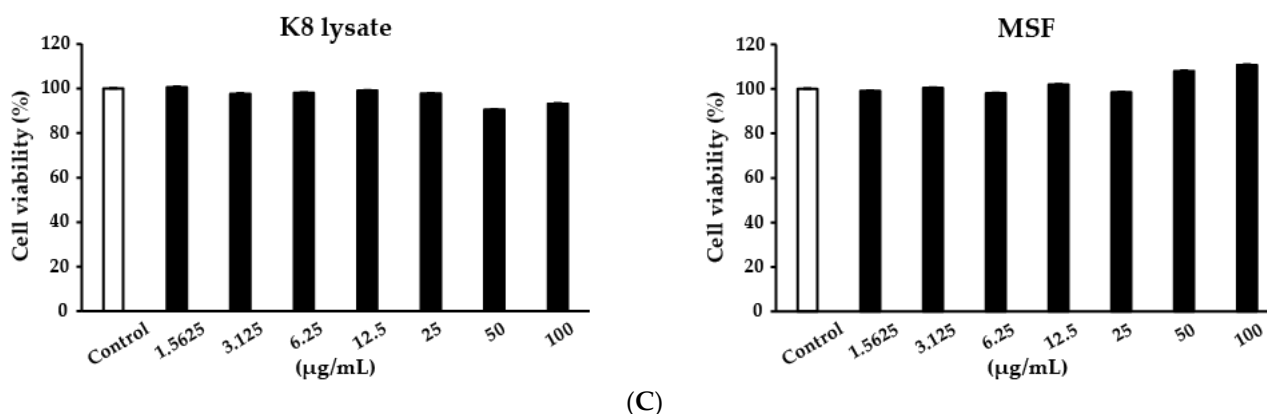
Figure 5. MSF inhibited the S. aureus -induced inflammation in THP1 cells. THP1 cells were pre-treated with MSF or K8 lysate (25, 50, and 100 µg/mL) for 1 h and then stimulated with heat-killed S. aureus ( 1 \times 10^8 CFU) for 24 h. (A) The expression of TNF- \alpha , IL-1 \beta , IL-6, and IL-8 was detected by qRT-PCR. (B) The protein levels of MAPKs and NF- \kappa B were checked by Western blot and Western blot quantification (the white bar is the phosphorylated form, and the black bar is the unphosphorylated form). (C) Cell viability of THP1 cells was tested by MTT assay with the indicated concentrations of MSF or K8 lysate. Data represent mean \pm SD from three independent experiments. # p < 0.05 , ## p < 0.01 , ### p < 0.001 vs. control. * p < 0.05 , ** p < 0.01 vs. model.
