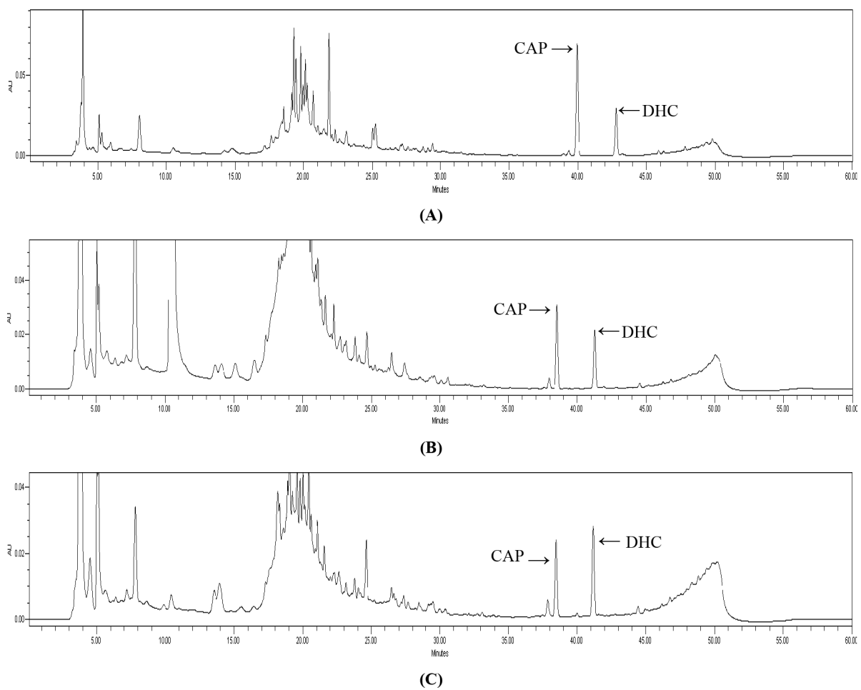
Fig. 4 HPLC chromatograms of capsicum samples 1 (A), 15 (B), and 20 (C)
