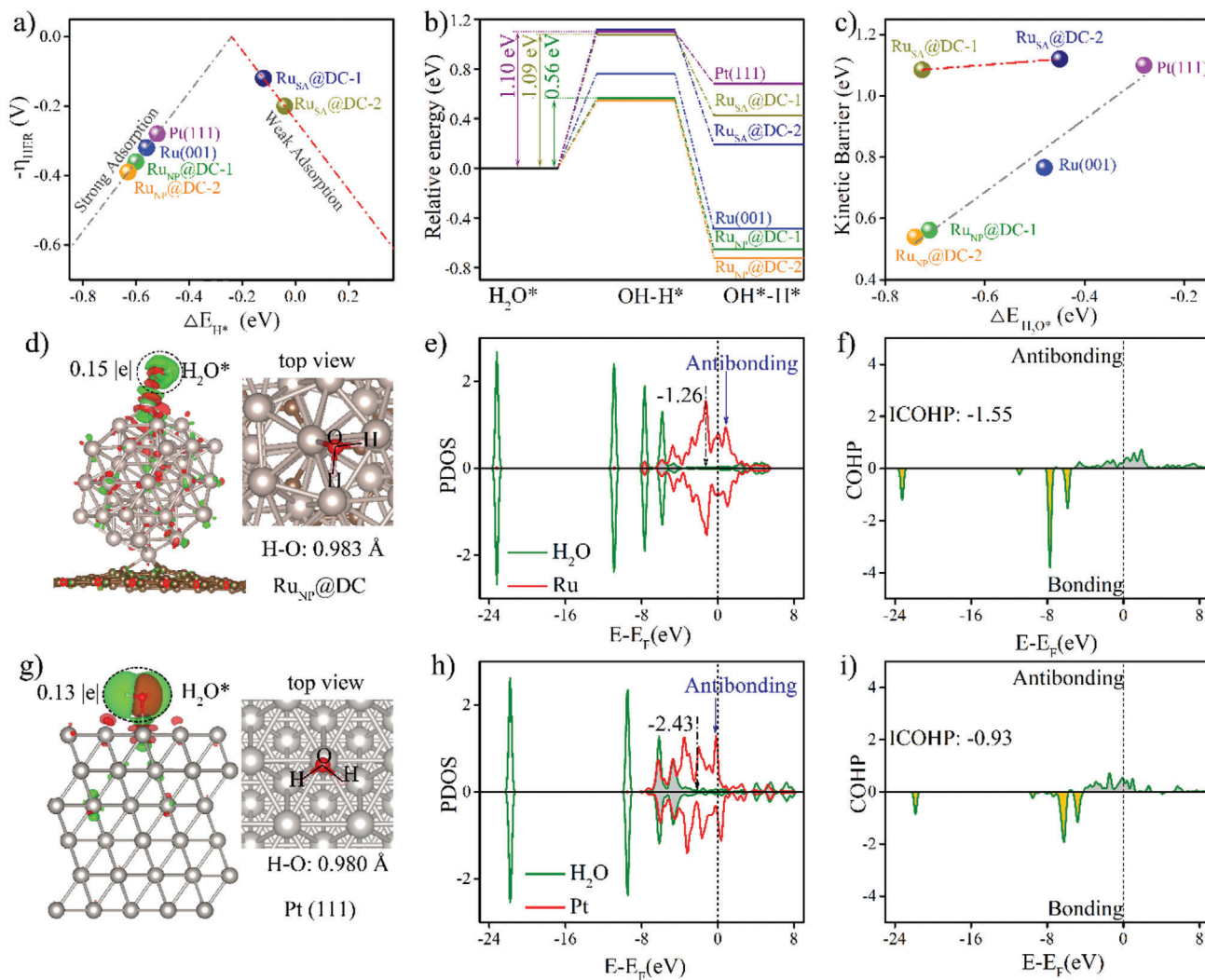
Figure 4. a) Volcano plot of theoretical \eta_{\text{HER}} versus \Delta E_{\text{H}^*} . b) Kinetic barrier of H 2 O dissociation for different models. c) Correlation between \Delta E_{\text{H}_2\text{O}^*} and energy barrier of H 2 O dissociation. d) Differential charge density distributions, e) PDOS, and f) COHP of active Ru atom for Ru NP @DC-1 and adsorbed H 2 O. g) Differential charge density distributions, h) PDOS, and i) COHP of active Pt atom for Pt(111) and adsorbed H 2 O. For differential charge density distributions, the green and red regions represent positive and negative charges, respectively.
