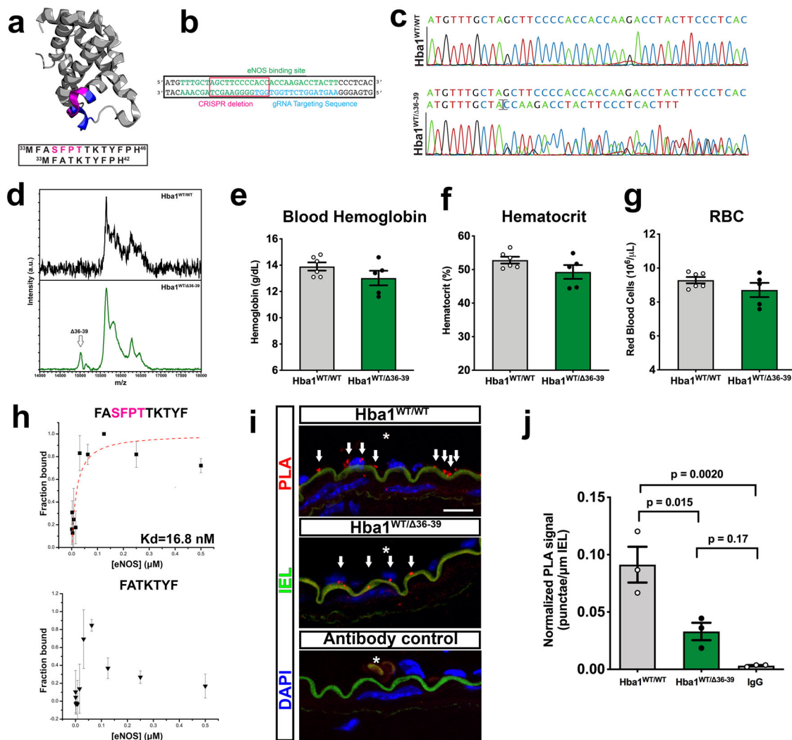
Fig. 4 | Disruption of alpha globin/eNOS interaction through the deletion of four residues in Hba1 . a A colored crystallographic model of alpha globin (from PDBid: 1ZSU) showing the residues previously shown to interact with eNOS (blue) surrounding four residues deleted in the Hba1 WT/Δ36-39 mouse model (magenta). The sequences for the proteins encoded by the Hba1 WT and Hba1 Δ36-39 alleles, including the deleted residues (magenta), are shown in the box below. b Using a guide RNA design (blue) targeting the eNOS binding region (green) resulted in an in-frame deletion of the nucleotides boxed in pink. This is confirmed by the chromatogram in c , which shows that the 12-nucleotide deletion scrambles downstream reading of the nucleotide sequence in NGS protocols. d The mutant protein is expressed, as seen in immunoprecipitation-coupled mass spectrometry. A peak corresponding to a protein with a molecular weight ~400 Da less than that of the dominant species is seen in hemoglobin captured from lysed red blood cells. e–g The blood hemoglobin content ( e ), hematocrit ( f ), and the number of red blood cells ( g ) are shown for the Hba1 WT/WT and Hba1 WT/Δ36-39 groups. h Results of fluorescence polarization assays for determining the binding of the mutant allele to eNOS, using an alpha globin mimetic peptide known to bind (top) and the Δ36–39 peptide (bottom). No binding affinity
