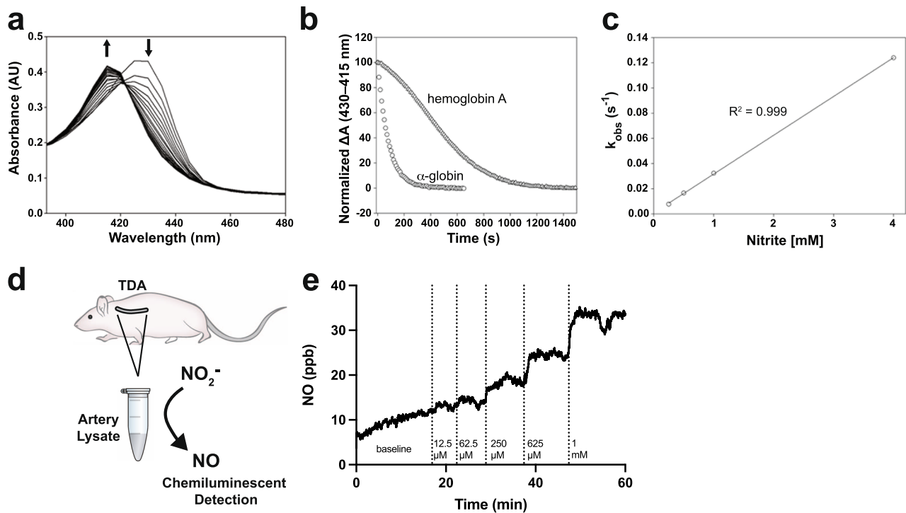
Fig. 2 | Alpha globin is a nitrite reductase. a Nitrite-induced optical changes to deoxyferrous alpha globin caused by NO gas formation and binding are reflected in the changing spectra over time. Sodium nitrite solution (1 mM) was added to deoxyferrous alpha globin (4 \mu\text{M} ), and spectra were recorded at 10-s intervals. b Example kinetic traces of ferrous-NO formation, as measured by the change in absorbance at 415 nm and 430 nm as a result of the reaction of alpha globin (circles) or hemoglobin A (triangles) and nitrite. c The observed rate constant for the formation of ferrous-NO from the reaction of (deoxy) alpha globin and nitrite across
