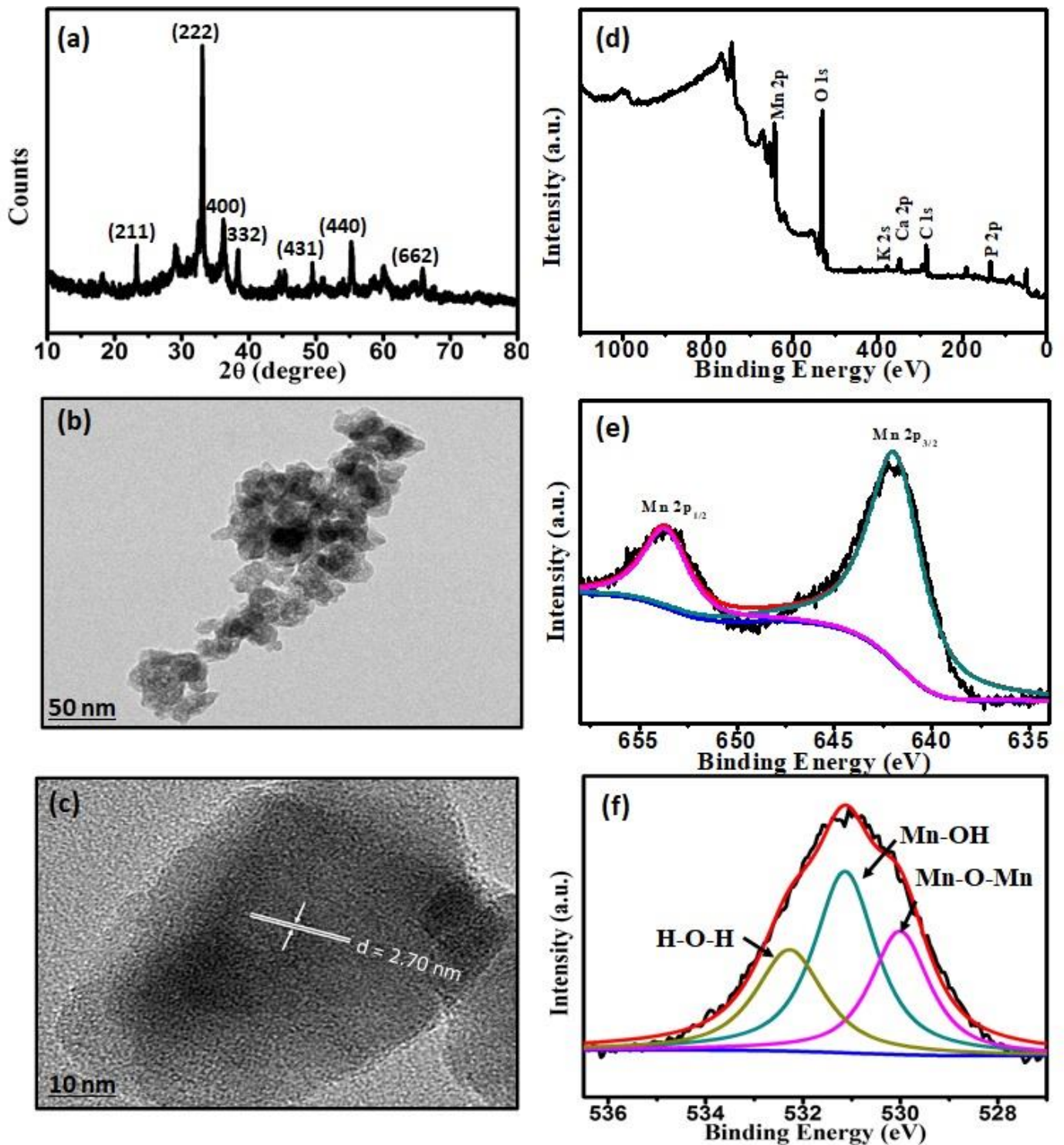
Figure 1. Characterization of MnO-NPs: (a) X-ray diffraction (XRD) pattern; (b) transmission electron microscopy (TEM) image; (c) high resolution (HR)-TEM image; (d) X-ray photoelectron spectroscopy (XPS) overview spectrum of MnO-NPs; (e,f) the narrow scan Mn 2p-electrons and O1s XPS spectrum of MnO-NPs, respectively.
