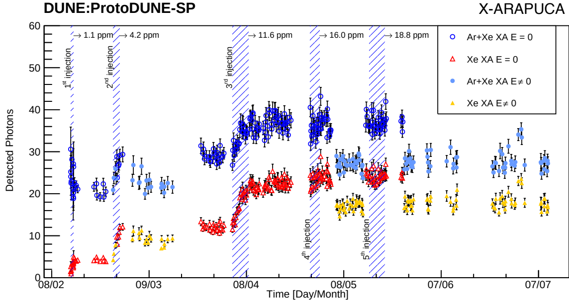
Figure 10. Light collected by the two X-ARAPUCA modules, in units of detected photons per trigger. Uncertainty bars are derived from statistical uncertainties evaluated on the spread of their distributions. Shaded areas represent xenon injection periods. The amount of collected light increases at each doping. Abrupt steps in the number of photons away from the injection periods correspond to the activation of the HV system of ProtoDUNE-SP and hence the presence of a non-zero electric field. Correspondingly, empty markers are results with no electric field, whereas filled markers correspond to runs with electric field (500 V/cm).
