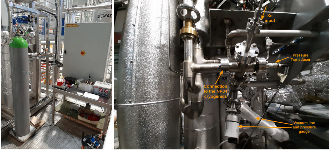
Figure 19. Left: the xenon bottle — on the scale — connected to the gas purifier, the mass flow-meter and the injection line. Right: detail of the UHV injection line equipped with vacuum/pressure monitoring devices and connected to the NP04 gas circulation system.
