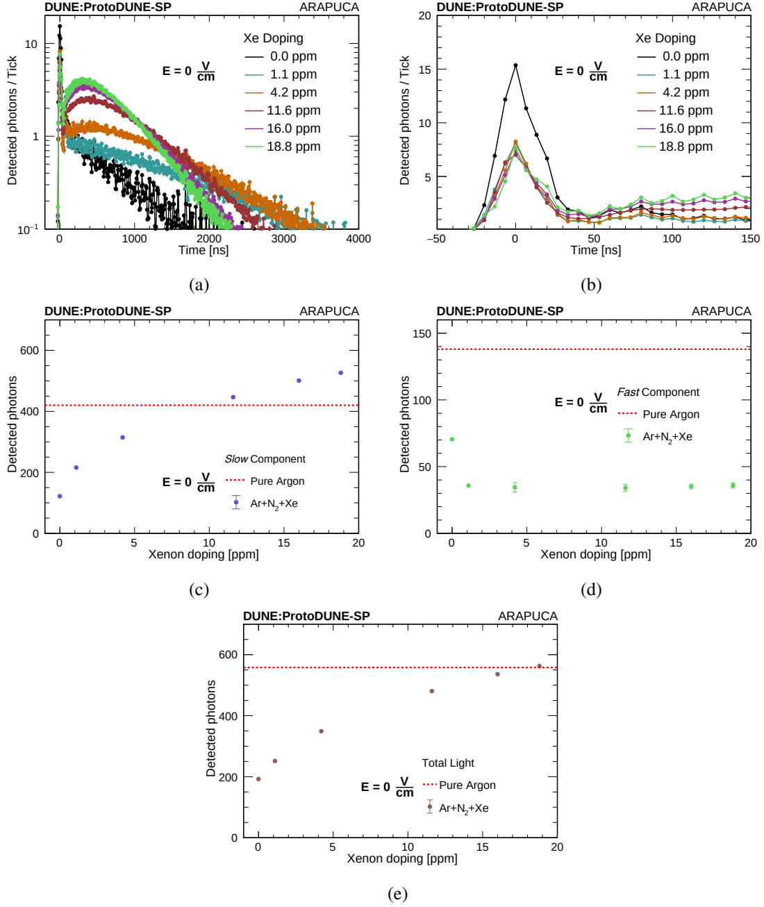
Figure 16. Data from ARAPUCA on the non-beam side TPC. Top row (a, b): deconvolved waveforms, changing in shape with increasing concentration of xenon; “0 ppm” data refer to argon polluted with nitrogen. Middle row: evolution of the slow (c) and fast (d) light components as a function of xenon concentration, in the nitrogen contaminated scintillation medium. Bottom row: evolution of the total detected light (e) as a function of xenon concentration, in the nitrogen contaminated scintillation medium.
