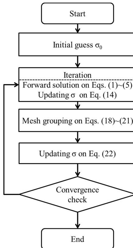
Fig. 1. Flowchart of Proposed Algorithm.
