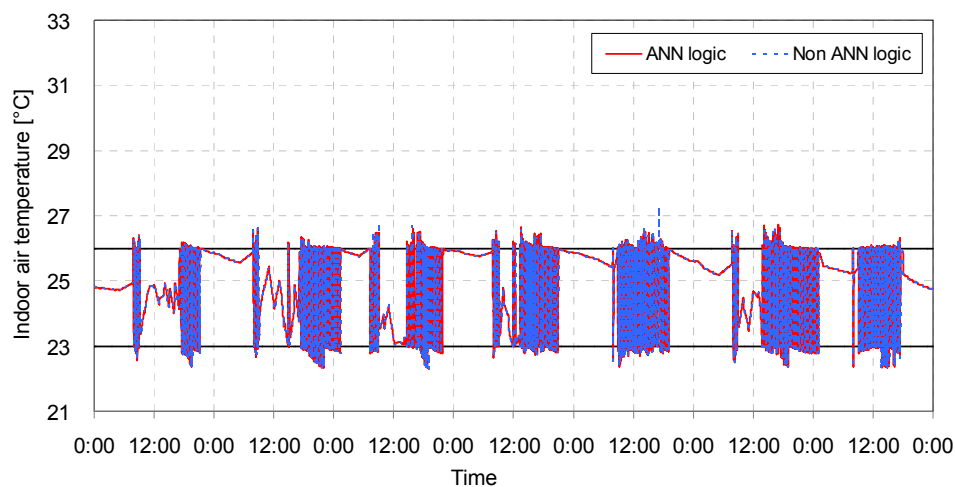
Figure 18. Profiles of the indoor air temperature for case 3 in summer (8–14 August). (Case 3—Opening at internal envelope: opened, Opening at external envelope: closed).
