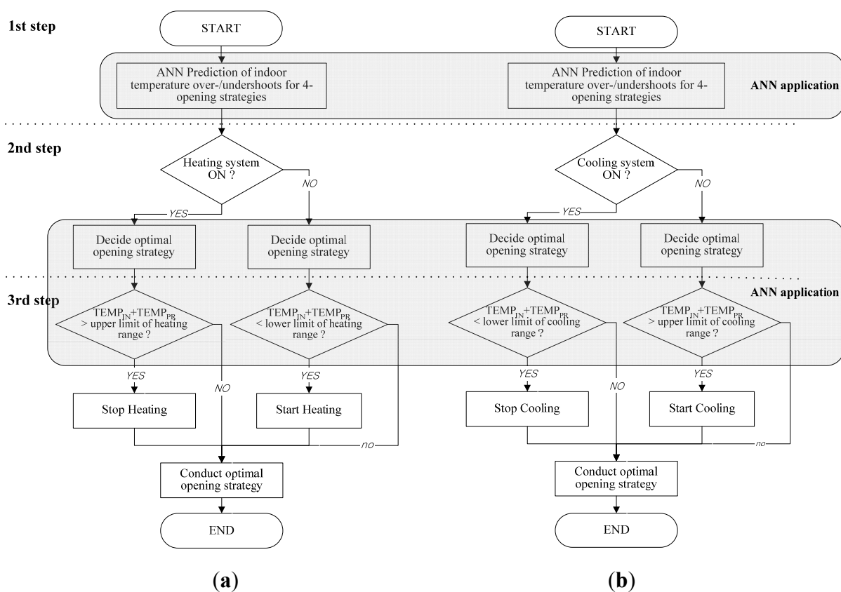
Figure 1. Integrated temperature control logic for buildings with double skin envelopes [1,2,8,10]. (a) Control logic for heating season; (b) Control logic for cooling season.
