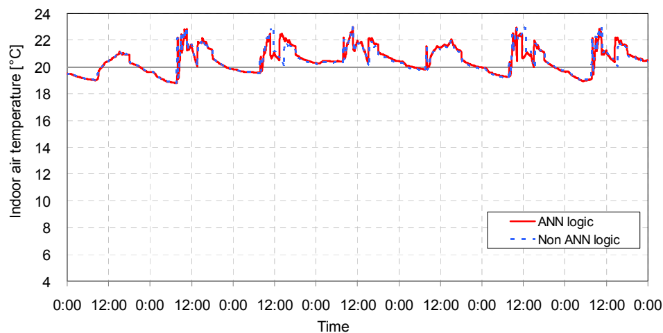
Figure 13. Profiles of the indoor air temperature for case 3 in winter (8–14 January). (Case 3—Opening at internal envelope: opened, Opening at external envelope: closed).
