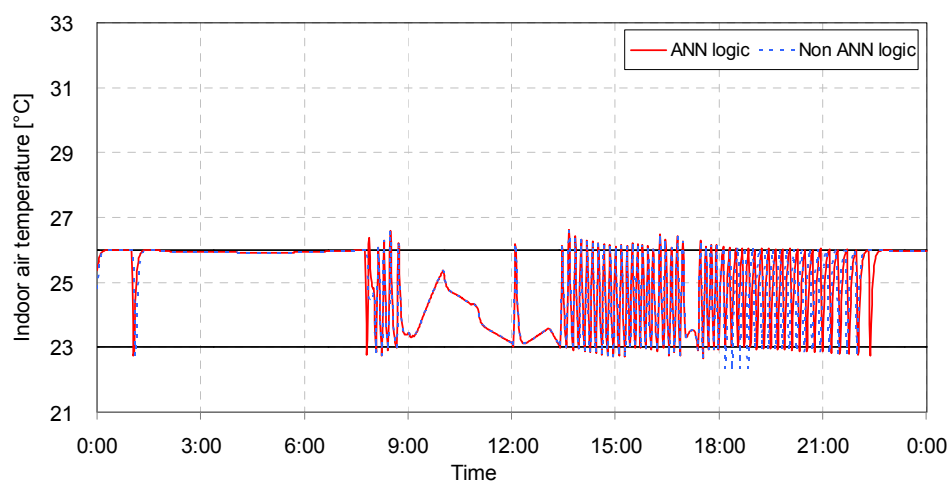
Figure 16. Profiles of the indoor air temperature for case 1 on a summer day (11 August only). (Case 1—Opening at internal envelope: closed, Opening at external envelope: closed).
