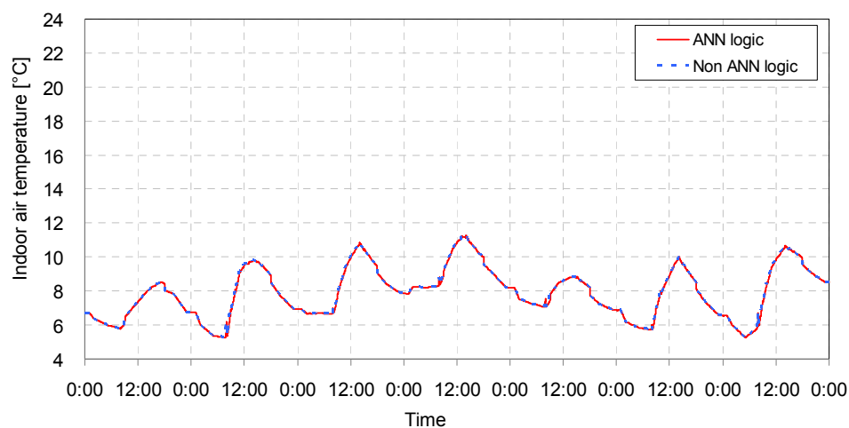
Figure 15. Profiles of the indoor air temperature for case 1 in summer (8–14 August). (Case 1—Opening at internal envelope: closed, Opening at external envelope: closed).
