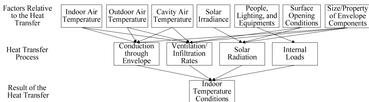
Figure 3. Influential factors in the variation of indoor temperature conditions.
