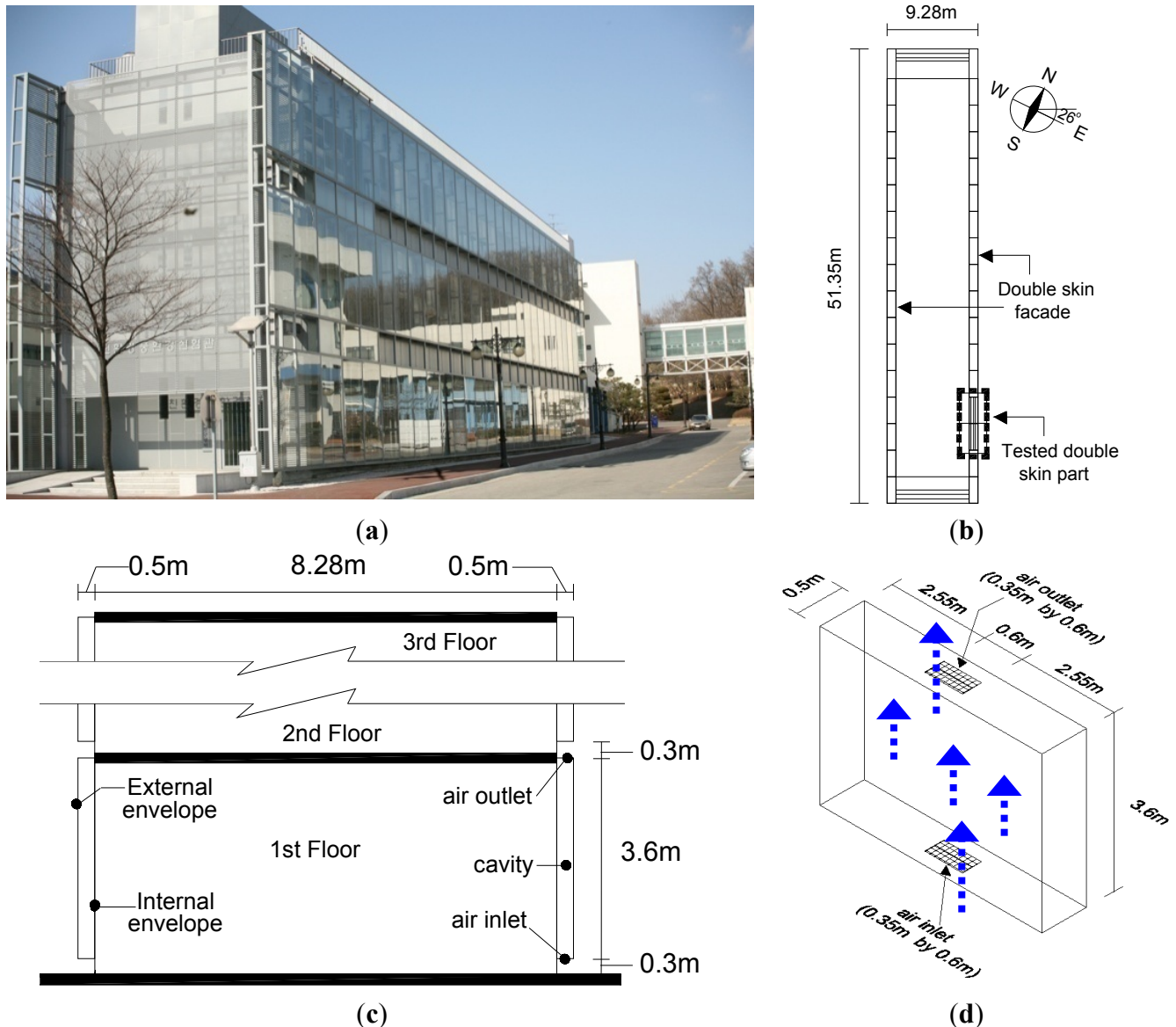
Figure 4. Layout of tested building and detailed description of cavity space. (a) View of building; (b) Layout of building; (c) Section of building; (d) Conceptual diagram of air flow in cavity.
