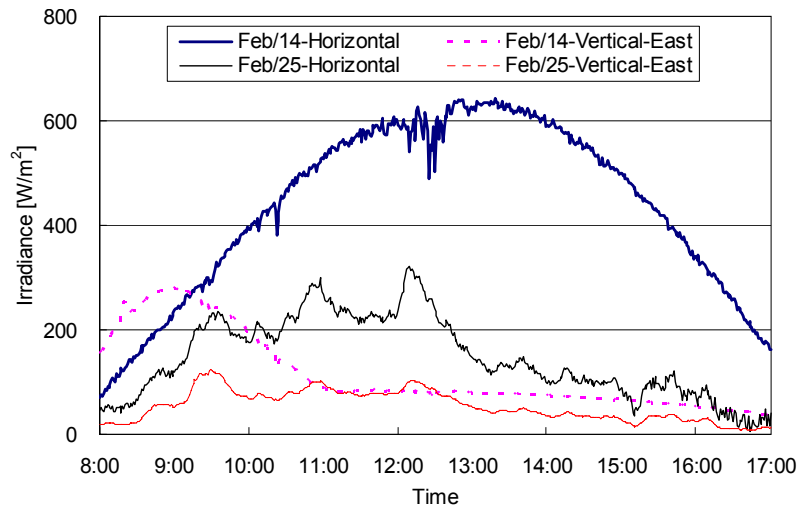
Figure 5. Variation of outdoor irradiance (East-facing, Clear and overcast sky).
