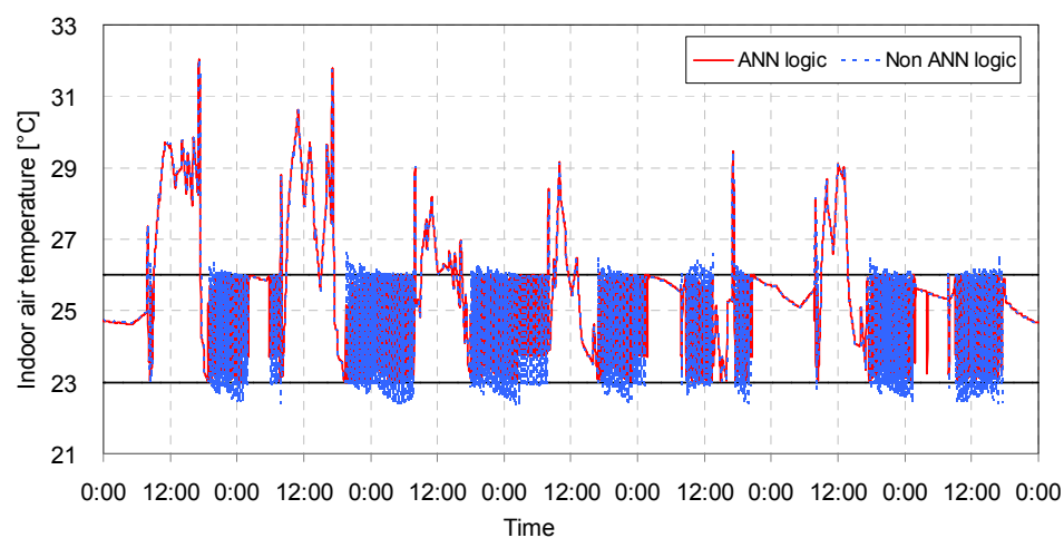
Figure 19. Profiles of the indoor air temperature for case 4 in summer (8–14 August). (Case 4—Opening at internal envelope: opened, Opening at external envelope: opened).
