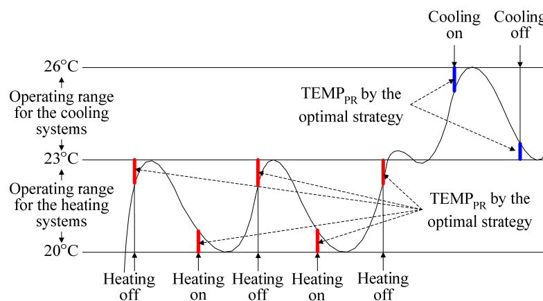
Figure 2. Conceptual profile of indoor temperature by ANN-based logic for heating and cooling season.
