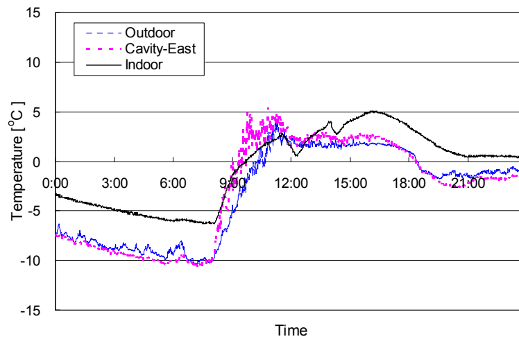
Figure 7. Variation of outdoor and cavity temperature (East-facing, 25 February, Overcast sky).
