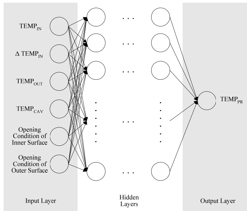
Figure 9. Structure of a new ANN model.
