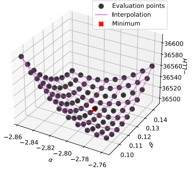
Figure 2. A plot visualizing the HAWC likelihood for an example source. The y-axis is the negative LLH. The negative LLH is evaluated around the best-fit model. For a log-parabola spectrum, we evaluate 50 points within \pm 5\sigma for \alpha and \beta around the minimum. For a power-law spectrum, we evaluate 300 points for spectral index within \pm 5\sigma . The negative log-likelihood was minimized over the gamma-ray flux for each point.
