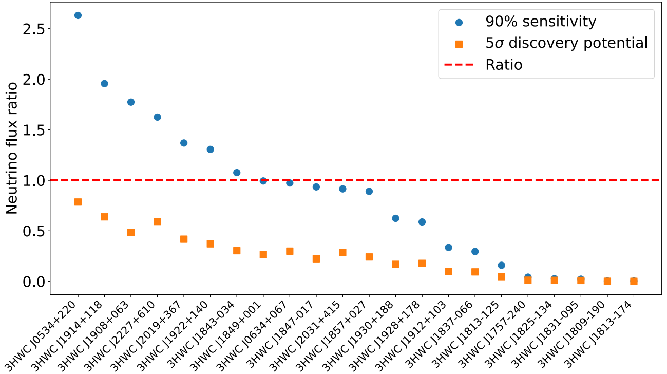
Figure 3. The ratio between the predicted neutrino flux and the sensitivity (blue dot) and 5\sigma discovery potential (orange rectangle) of the analysis. The sources above the red dashed line are the sources that are likely to be detected by IceCube if they are hadronic sources. The plot is ordered by the sensitivity ratio.
