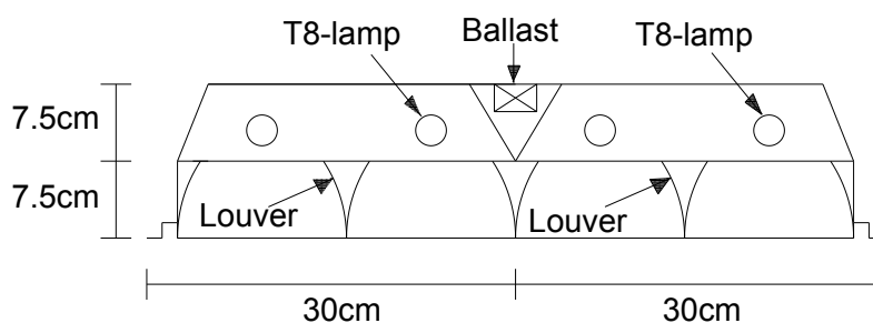
Figure 2. Section of fluorescent lighting fixture.
