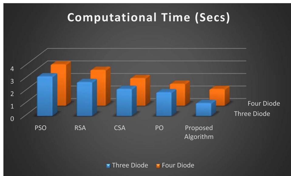
Figure 6. Computational time of both diode.
