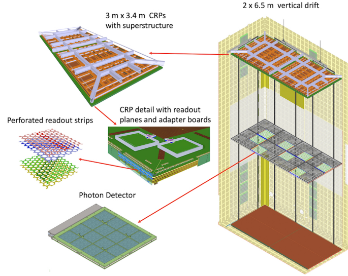
Figure 8. Schematic of the vertical drift FD2 concept with PCB -based charge readout. Corrugations on cryostat wall shown in yellow; PCB -based CRPs (brown, at top and bottom with superstructure in gray for top CRPs); cathode (violet, at mid-height with openings for photon detectors); field cage modules (white) hung vertically around the perimeter (the portions near the anode planes are 70% optically transparent); photon detectors (light green at right), placed in the openings on the cathode and on the cryostat walls, around the perimeter in the vertical regions near the anode planes. Reproduced from [60]. The Author(s). CC BY 4.0.
