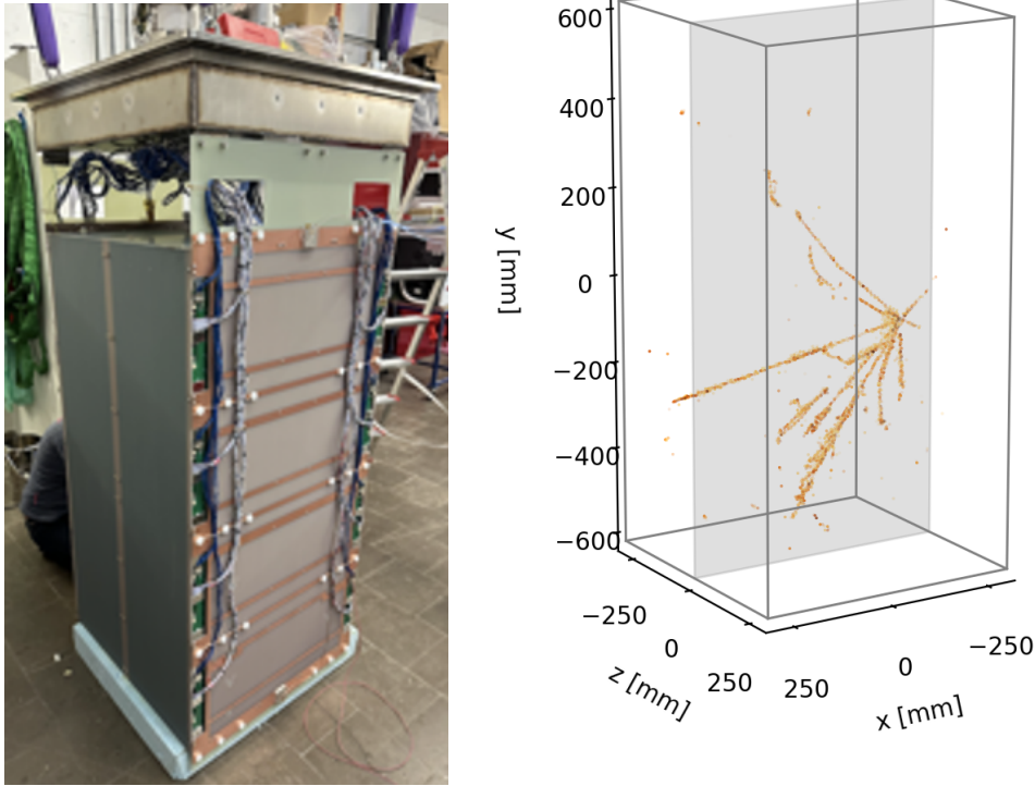
Figure 17. Left: a photograph of one of the four ton-scale LArTPC modules for the 2x2 Demonstrator, a prototype of the DUNE ND . Right: an example cosmic ray imaged in true 3D using a 102,400-channel LArPix-v2 system in this module (right).
