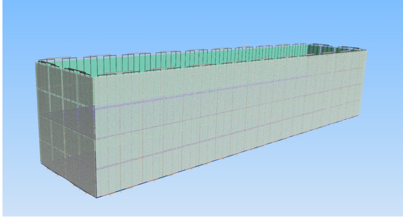
Figure 12. A bird’s-eye view of the field cage with integrated large-area photon detection system, APEX . The field cage structure is constructed of modules vertically stacked in groups of four hanging around the LAr drift volume perimeter from the top.
