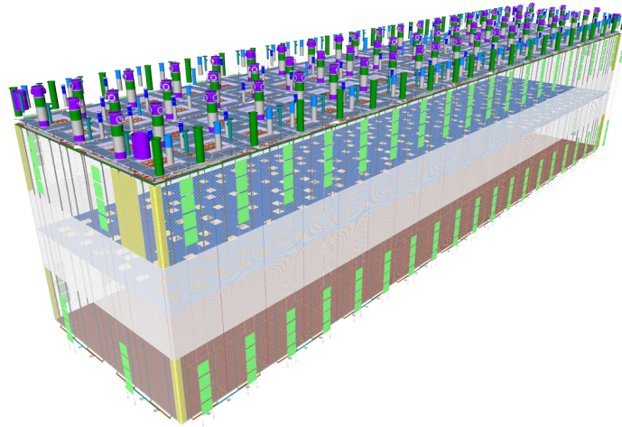
Figure 9. Perspective view of the vertical drift FD2 detector. Reproduced from [60]. The Author(s). CC BY 4.0.
