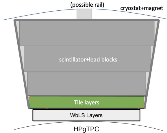
Figure 32. An upstream segment of the GArTPC ECAL , with the beam is pointing downward. The THEIA layers constitute the most downstream portion of the ECAL , and particles produced in these layers via neutrino interactions are tracked in the downstream HPgTPC .
