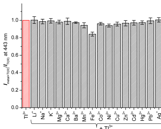
Fig. 2 Changes in fluorescence intensity ratio ( I_{\text{metal+Tl(m)}}/I_{\text{Tl(m)}} ) of TP-1 at 443 nm in the presence of coexisting metal ions. [ TP-1 ] = 5.0 \mu\text{M} , [Tl 3+ ] = [M n+ ] = 50 \mu\text{M} , in a pH 4.8 acetate buffer solution (10 mM) containing 1% (v/v) DMF. \lambda_{\text{ex}} = 309 nm.
