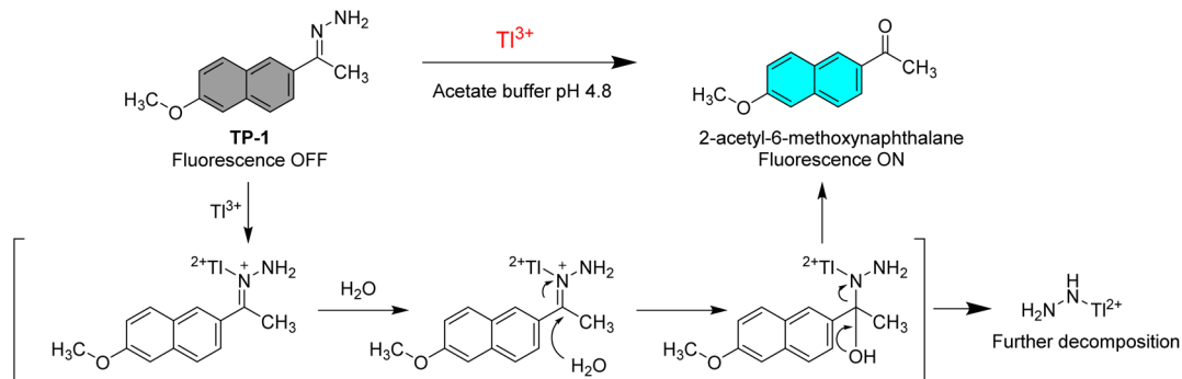
Scheme 2 Suggested Ti^{3+} sensing mechanism of TP-1.
