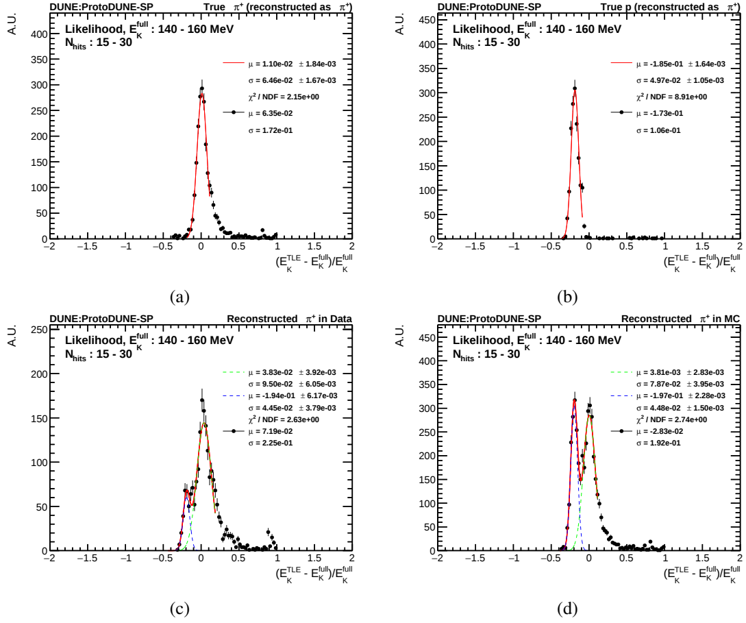
Figure 13. Example distributions of the fractional energy residual using range-based E_K as reference. Results come from reconstructed charged pions with 15 to 30 hits and E_K^{\text{full}} from 140 MeV to 160 MeV. Top plots show results for MC true pions (a) and true protons (b). Bottom plots show results using all reconstructed charged pions for data (c) and the MC sample (d), where green and blue Gaussian functions represent charged pion and proton contributions, respectively.
