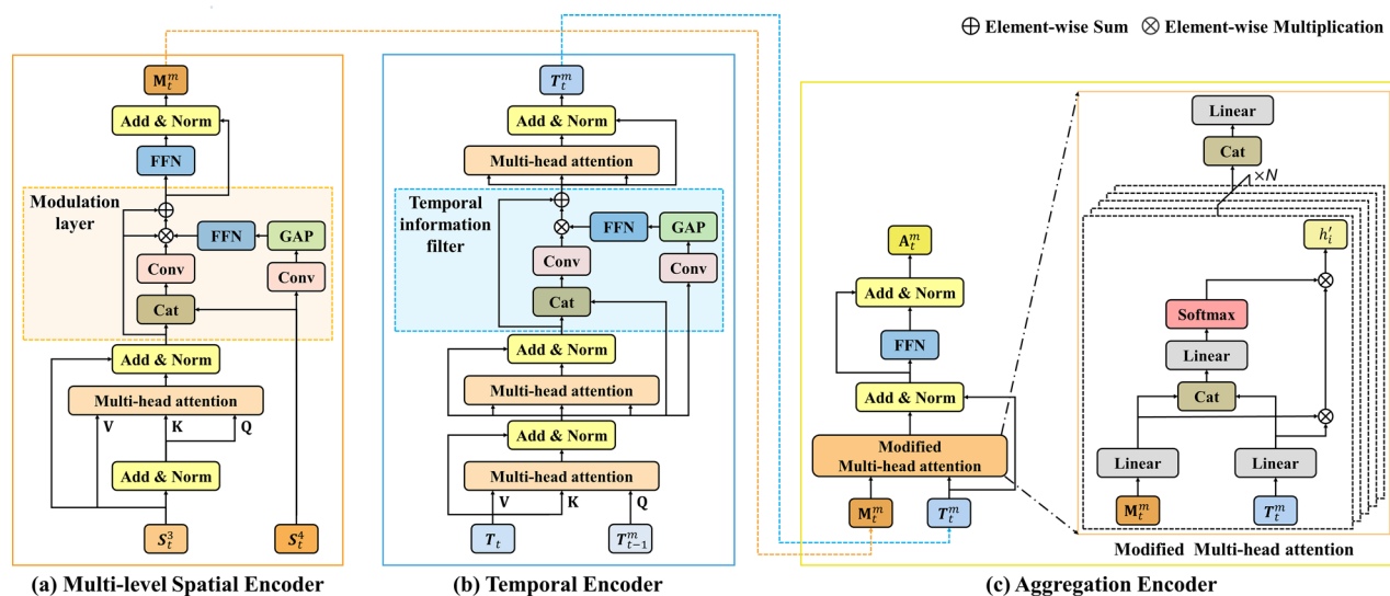
Fig. 3. Architecture of the proposed transformer encoder. The proposed encoder consists of three components: a multi-level spatial encoder, a temporal encoder, and an aggregation encoder.
