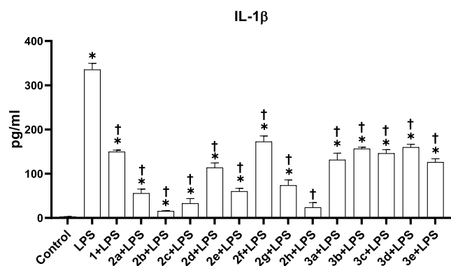
Figure 3. Inhibitory effect of active compounds on IL-1 \beta production. RAW 264.7 cells were pretreated with 20 \mu\text{M} active compounds for 2 h, followed by 100 ng/mL LPS for 24 h. An IL-1 \beta ELISA kit was used to check IL-1 \beta production in the media of the RAW 264.7 cells. Values are presented as means \pm standard errors. * p < 0.05 compared with the control, † p < 0.05 compared with LPS alone.
