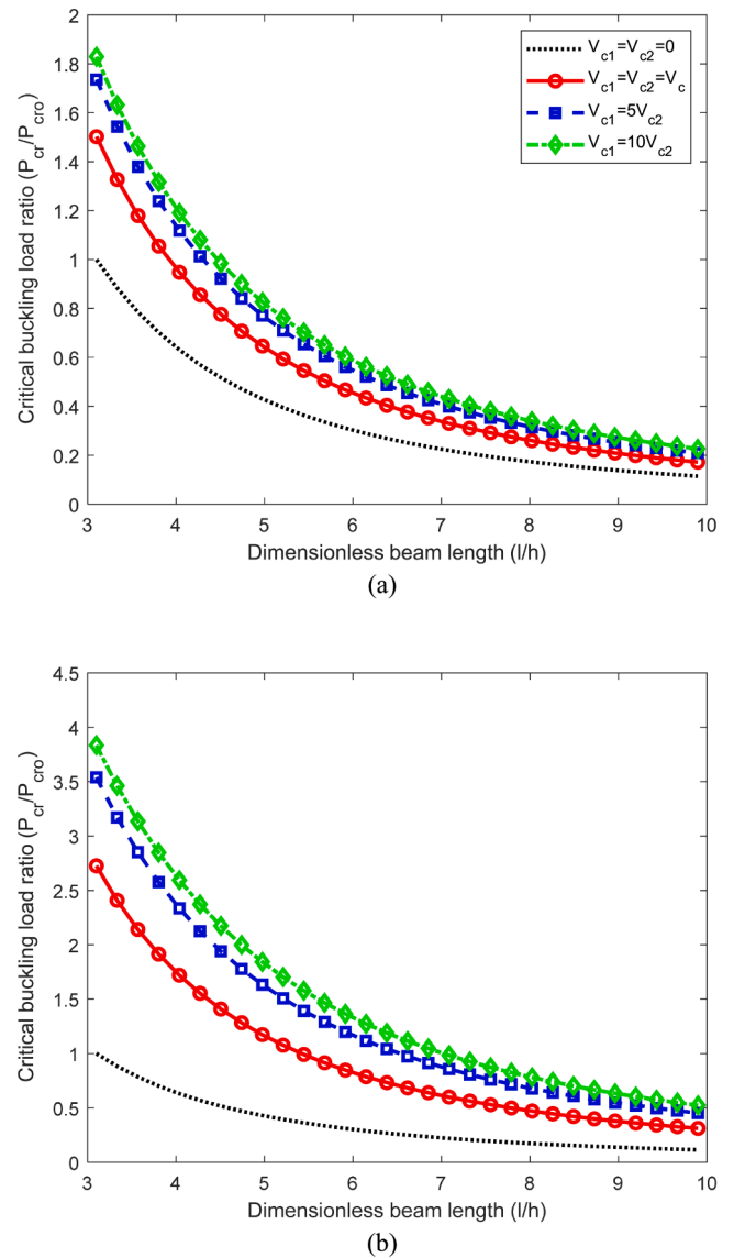
Fig. 3. Effect of CNTs on critical buckling load of CNT-reinforced FG composite beams. (a) V_c = 1.5\% and (b) V_c = 5.0\% ( P_{cr0} is the critical buckling load of the beam with no CNTs at beam length l = 3.1 h ).
