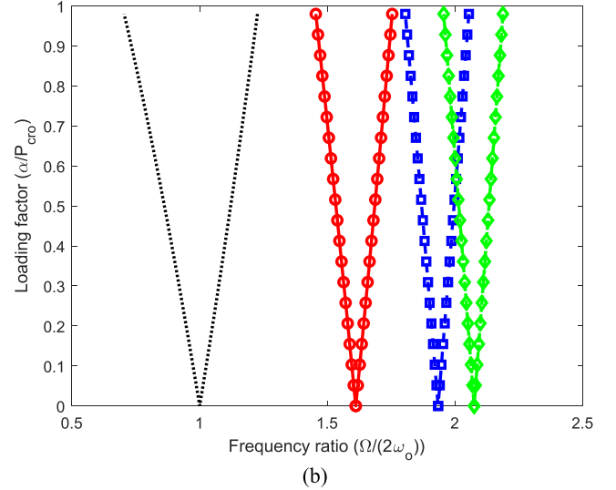
Fig. 5. The dynamic instability zones of CNTs-reinforced FG composite beams. (a) V_c = 1.5\% and (b) V_c = 5.0\% ( l = 8h , \omega_o and P_{cro} are the fundamental frequency and critical buckling load of the beam with no CNTs).
