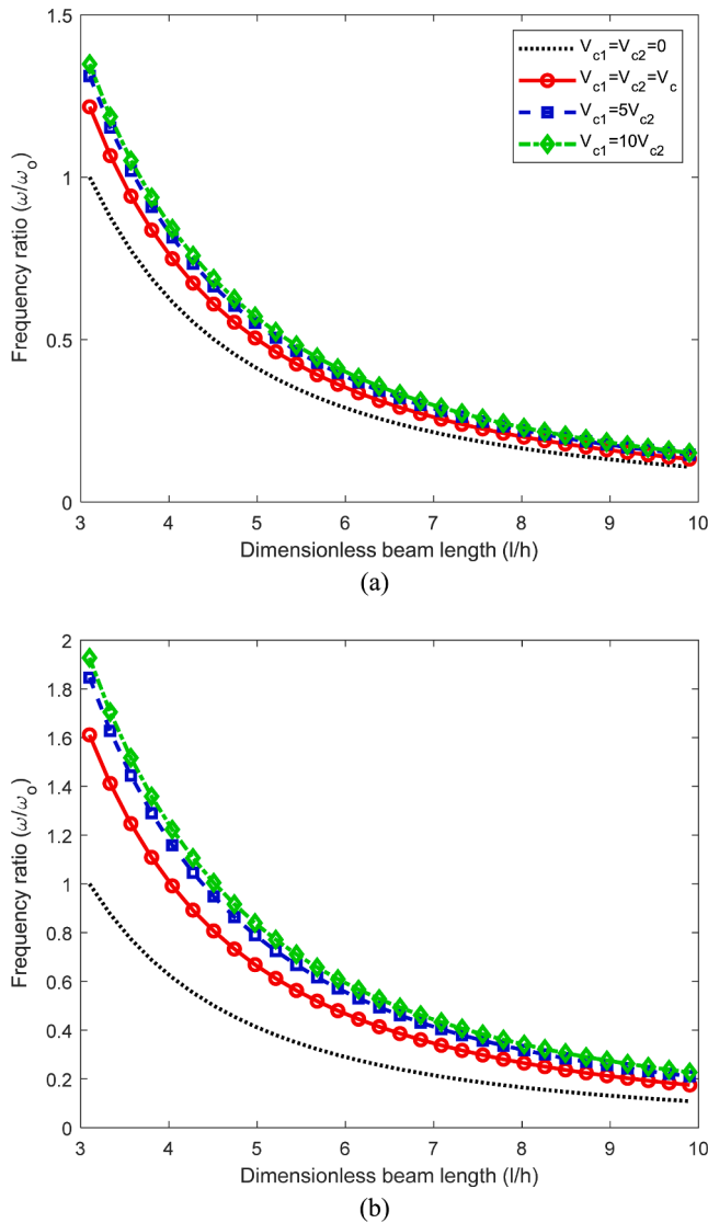
Fig. 2. Effect of CNTs on fundamental frequency of CNTs-reinforced FG composite beams. (a) V_c = 1.5\% and (b) V_c = 5.0\% ( \omega_0 is the fundamental frequency of the beam with no CNTs at beam length l = 3.1 h ).
