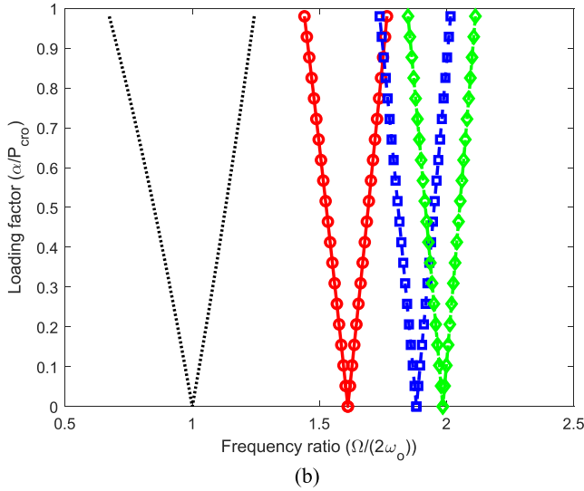
Fig. 4. The dynamic instability zones of CNTs-reinforced FG composite beams. (a) V_c = 1.5\% and (b) V_c = 5.0\% ( l = 4h , \omega_o and P_{cro} are the fundamental frequency and critical buckling load of the beam with no CNTs).
