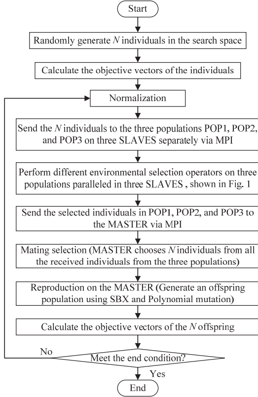
Fig. 2 The flowchart of PMEAs
