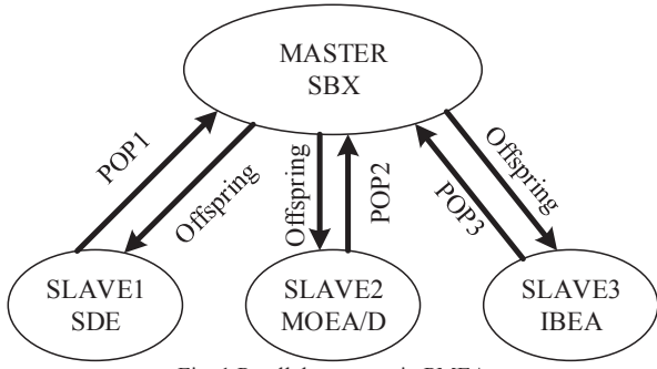
Fig. 1 Parallel structure in PMEAs
