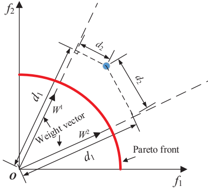
Fig.4 Illustration of the distance d_1 and d_2 .
