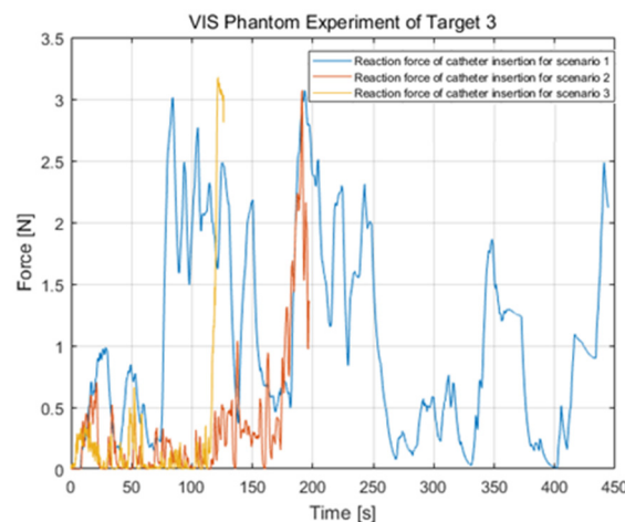
Figure 17. Reaction force in the three different scenarios for Target 3.
