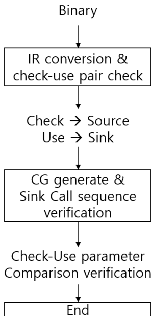
Fig. 7. Vulnerability detection process between different functions
