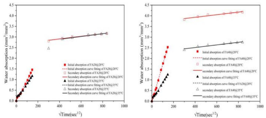
Figure 2. Cumulative water absorption of the pastes cured after 28d for (a) FA20 and (b) FA40
