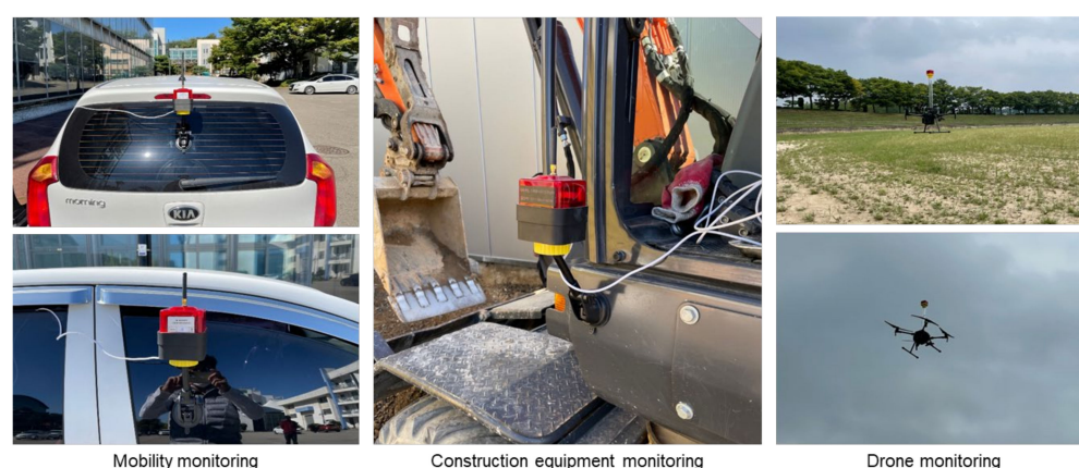
Figure 2. Mobile installation of CPMS.
