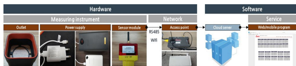
Figure 7. CPMS network composition.
