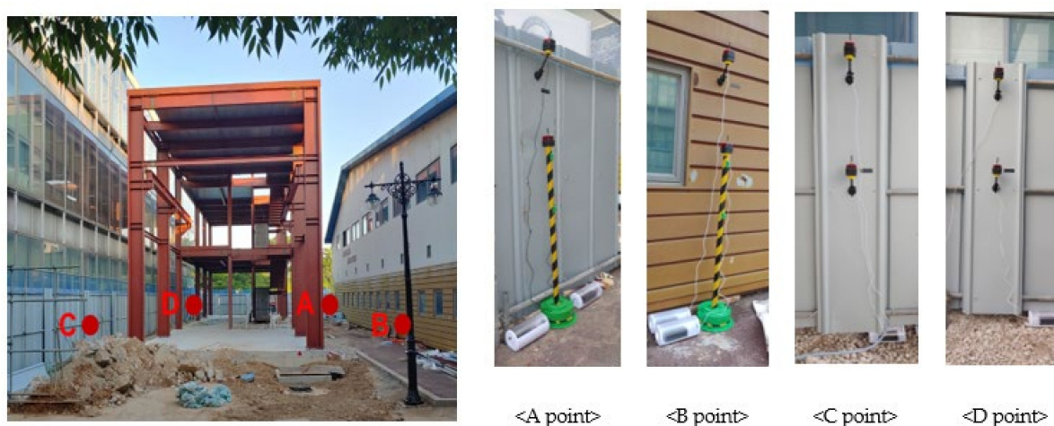
(a) Installation nodes of the construction site measuring instruments
