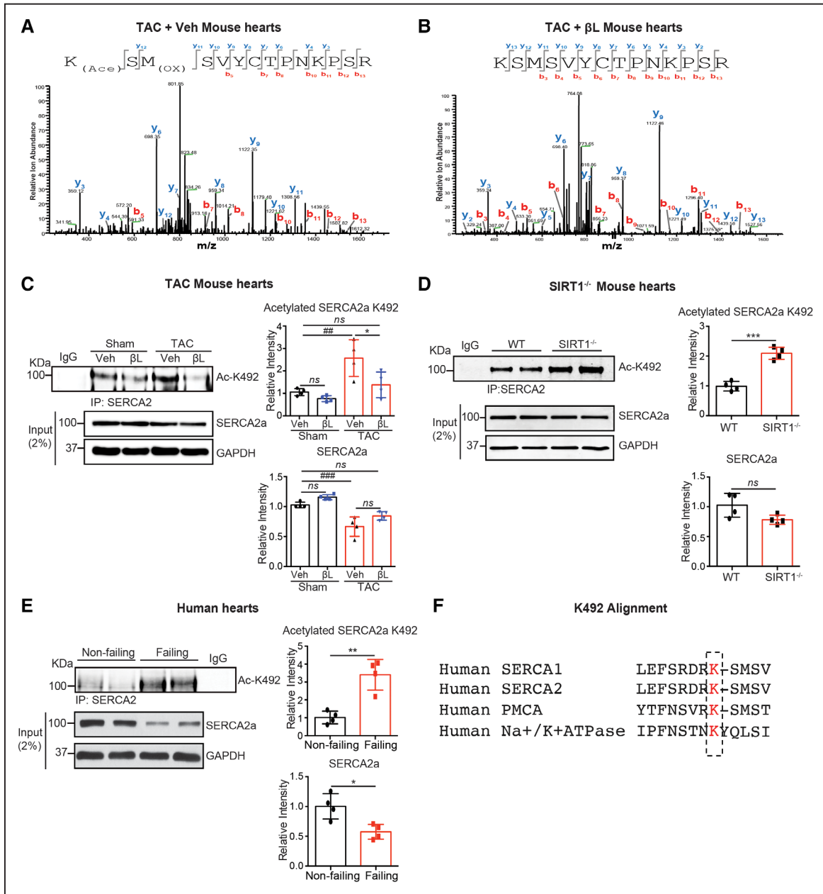
Figure 6. Acetylation of K492 on SERCA2a (sarco-endoplasmic reticulum \text{Ca}^{2+} -ATPase) is increased in failing and SIRT1 (sirtuin 1) knockout hearts. A and B , Representative MS/MS spectra of tryptic peptides of SERCA2a at K492 identified in transverse aortic constriction (TAC) mouse hearts treated with vehicle (Veh) or \beta L ( \beta -lapachone). A , Acetyl-Lys peptide \text{K}_{\text{Ac}}\text{SM}_{\text{OX}}\text{SVYCTPNKPSR} (residues 492–505) was detected in heart extracts from TAC mice. B , Lys peptide \text{KSMSVYCTPNKPSR} (residues 492–505) was detected in heart extracts from TAC mice treated with \beta -lap (TAC+ \beta L). \text{K}_{\text{Ac}} : acetyl-lysine; \text{M}_{\text{OX}} : oxidized methionine. C , Levels of K492 acetylation of SERCA2a were elevated in TAC-induced failing mouse hearts, as determined by a specific antiacetyl-K492 antibody. The representative immunoblots were presented. Graphs show means \pm SD, with each data point representing 1 heart sample. n=4 per each group. * P<0.05 vs \beta -lap treatment and ### P<0.01 ; ### P<0.001 vs Sham+Veh by 1-way ANOVA. D , Acetylation levels of SERCA2a at K492 were elevated in SIRT1 -/- mouse hearts. The representative immunoblots were presented. Graphs show means \pm SD, with each data point representing 1 heart sample. n=4 per each group. *** P<0.001 vs wild-type (WT) by unpaired t test. E , Acetylation levels of SERCA2a at K492 were increased in human failing hearts. The representative immunoblots were presented. Graphs show means \pm SD, with each data point representing 1 heart sample. n=4 per each group. * P<0.05 ; ** P<0.01 vs nonfailing by unpaired t test. F , Amino acid sequence alignment of different members of the human P-ATPase family of proteins showing high degree of conservation of K492 (K492 and homologous lysine residues are highlighted in red). Ac-K492 indicates acetylated K492; Acetyl-Lys, anti-acetylated lysine antibody; IP, immunoprecipitation; MS/MS, tandem mass spectrometry; ns indicates not significant; and PMCA, plasma membrane \text{Ca}^{2+} ATPase.
