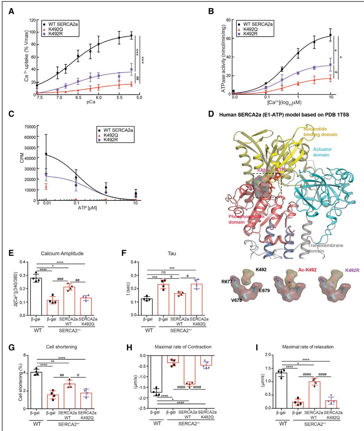
Figure 7. Acetylation at K492 plays a critical role in regulating SERCA2a (sarco-endoplasmic reticulum Ca 2+ -ATPase) activity. A , The calcium uptake, (B) ATPase activity, and (C) ATP-binding assays of SERCA2a in microsomal fractions isolated from HEK293 (human embryonic kidney) cells transfected with wild-type (WT) or mutant (K492Q or K492R) forms of SERCA2a (normalized to expression levels of SERCA2a). Data are represented as the mean±SD of n=3 experiments. *P<0.05; ***P<0.001 vs WT SERCA2a and #P<0.05; ###P<0.01 vs K492R SERCA2a by paired t test. D , K492 acetylation site is located in the ATP-binding pocket of SERCA2a. Cartoon representation of SERCA2a based on the crystal structure of SERCA1a (PDB: 1T5S). The phosphorylation domain, nucleotide-binding domain, and actuator domain are shown in salmon, yellow, and cyan, respectively. The transmembrane domain is shown in grey. K492 (pink) is located within the nucleotide-binding domain adjacent to the ATP molecule (red). Close-up views of K492, acetylated K492 (Ac-K492), and nonacetylated K492 mutant (K492R) relative to the phosphorylation domain are shown on the bottom. E through I , Overexpression of the acetyl-mimicking mutant (K492Q) of SERCA2a showed contractile dysfunction in adult cardiomyocytes isolated from SERCA2 -/- mice. Adult ventricular cardiomyocytes were isolated from SERCA2 -/- mice and infected with Ad-WT SERCA2a, Ad- K492Q SERCA2a, or Ad-β-gal (β-galactosidase as a negative control). Adult mouse cardiomyocytes (ACMs) isolated from WT mice infected with Ad-β-gal served as control. The contractile response of SERCA2a restoration in SERCA2 -/- ACMs was assessed by calcium amplitude (E) , decay time constant (tau; F ), peak shortening (G) , maximal rate of contraction (H) , and maximal rate of relaxation (I) using a video-based edge-detection system (IonOptix, Inc. Milton, MA) 24 h after infection of ACMs with adenovirus (50 MOI of each virus). n=4. Graphs show means±SD, with each data point was represented a mean average of 15 ACMs isolated from 1 heart sample. *P<0.05; **P<0.01; ***P<0.001; ****P<0.0001 vs WT+β-gal and #P<0.05; ###P<0.001; ####P<0.0001 vs SERCA2 -/- SERCA2a-WT by 1-way ANOVA. Ad indicates adenovirus; CPM, counts per minute; MOI, multiplicity of infection; ns, not significant pCa, calcium concentration; and PDB, Protein Data Bank.
