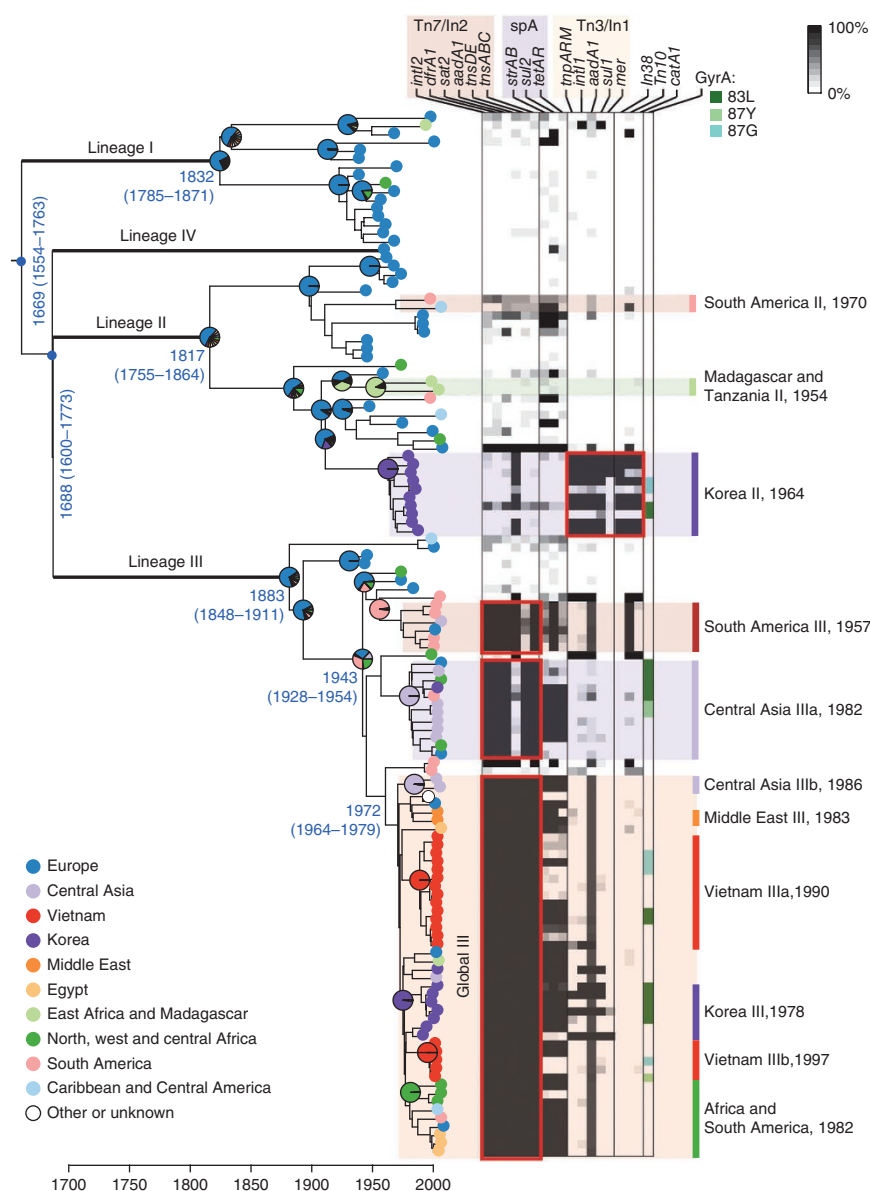
Figure 1 Bayesian maximum clade credibility phylogeny for S. sonnei . Left, branches defining major lineages are shown in bold (each with 100% posterior support). Pie charts indicate maximum-likelihood estimates for geographic origin of major nodes (legend at bottom). Divergence dates (median estimates and 95% HPD) are given in blue for major nodes. Right, the distribution of antimicrobial resistance determinants is indicated in the heatmap, reflecting the percentage of bases in each gene sequence that are covered by reads from each isolate (legend at top). GyrA mutations 83L, 87Y and 87G are indicated by color (inset legend). Likely MDR acquisition events are highlighted with red boxes. Geographically localized clonal expansions are highlighted and labeled with their median estimated divergence dates.
