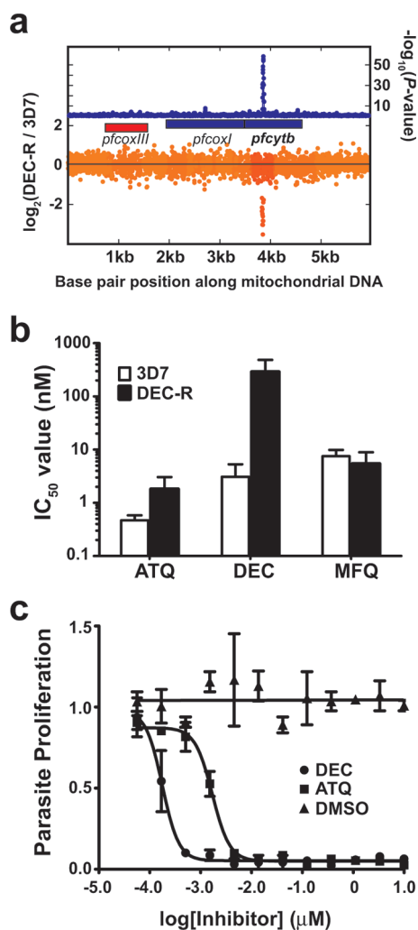
Figure 2. Decoquinat has a resistance and activity profile similar to that of atovaquone. (a) The -\log(P\text{-value}) for hybridization differences (z-test; blue line) is shown for pfcytb and flanking DNA. The spike is characteristic of a detected SNP. Below the gene model, the loss of hybridization resulting from the polymorphism was visualized probe-by-probe by plotting the \log_2 ratio of probe intensities in the decoquinat-resistant line versus the parental 3D7 line. (b) The IC_{50} values for atovaquone (ATQ), decoquinat (DEC), and mefloquine (MFQ) are shown for the parental 3D7 strain (white bars) and the DEC-R line (black bars). Statistically significant differences between IC_{50} values of the parental 3D7 line and the DEC-R line were calculated by a two-tailed unpaired t test: *P < 0.001 . (c) Inhibition curves of decoquinat (circles) and atovaquone (squares) against P. yoelii sporozoites in human liver cells. The IC_{50} values were calculated using a nonlinear regression curve fit. Atovaquone was determined to have an IC_{50} value of 1.7 nM, whereas decoquinat had activity equivalent to that of atovaquone at one log lower inhibitor concentration ( IC_{50} = 177 pM). DMSO had no effect on the culture. IC_{50} values for all experiments are represented as means \pm SD and were calculated from at least two independent experiments performed in duplicate.
