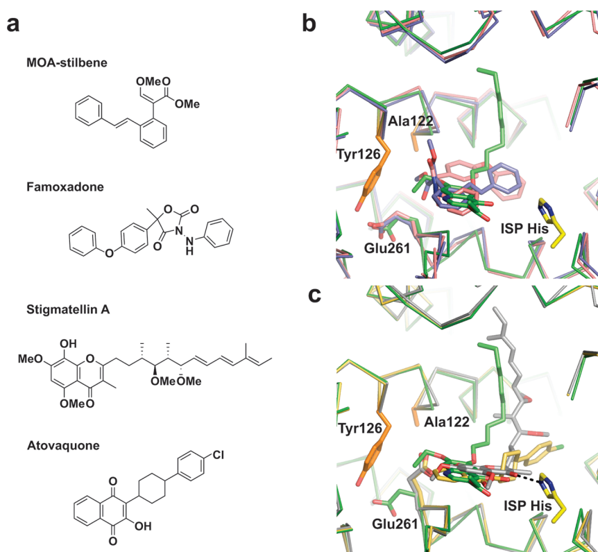
Figure 3. Decoquinone is predicted to be a class Ia inhibitor of the Q_o site in cytochrome b . (a) The chemical structures of putative Q_o site inhibitors are shown. (b) The docking results between decoquinone (green) and the P. falciparum cytochrome b homology model were superimposed onto the cytochrome b subunit of bovine cytochrome bc 1 complex co-crystallized with class Ia inhibitors MOAS (slate blue; PDB ID = 1SQQ) and famoxadone (pink; PDB ID = 1L0L) with a rmsd of 0.389 and 0.355 Å, respectively. The resistance-conferring mutations at residues Ala122 and Tyr126 (orange) are shown in the homology model (green). The histidine from the neighboring Rieske ISP subunit is labeled and shown in yellow. The noncarbon atoms are displayed with conventional colors: oxygen in red and nitrogen in blue. (c) Superposition of the decoquinone and atovaquone (yellow) energy minimization results with the cytochrome b subunit of bovine cytochrome bc 1 complex co-crystallized with the class Ib inhibitor stigmatellin A (gray; PDB ID = 1SQX). The rmsd between models is 0.219 Å. The hydrogen bond between stigmatellin A and the histidine residue from the Rieske ISP subunit is depicted as a dashed line. The figure was generated using Pymol software.
