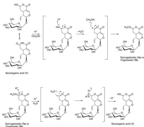
FIGURE 4 Proposed mechanism of (a) conversion of secologanic acid (1) into epivogeloside (1a) or vogeloside (1b), or (b) vice versa
