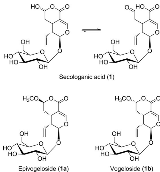
FIGURE 1 Chemical structures of secologanic acid ( 1 ) and its unwanted products, epivogelosiide ( 1a ) and vogelosiide ( 1b )
