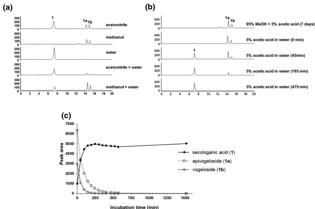
FIGURE 3 Conversion of secologanic acid (1) into epivogeloside (1a) or vogeloside (1b) or vice versa. (a) Conversion of secologanic acid (1) into epivogeloside (1a) or vogeloside (1b) in acetonitrile or methanol solution. (b) Conversion of epivogeloside (1a) or vogeloside (1b) into secologanic acid (1) in an acidic aqueous solution. (c) Conversion rate of epivogeloside (1a) or vogeloside (1b) into secologanic acid (1) in aqueous solution correspondence to the incubation time
