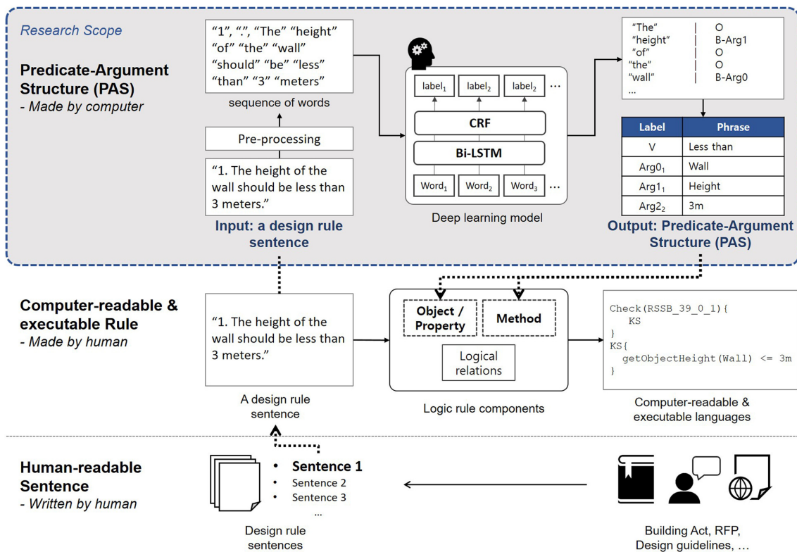
Figure 8: Deep learning and NLP-based PAS extraction in the rule-making process (extended from Fig. 1).
