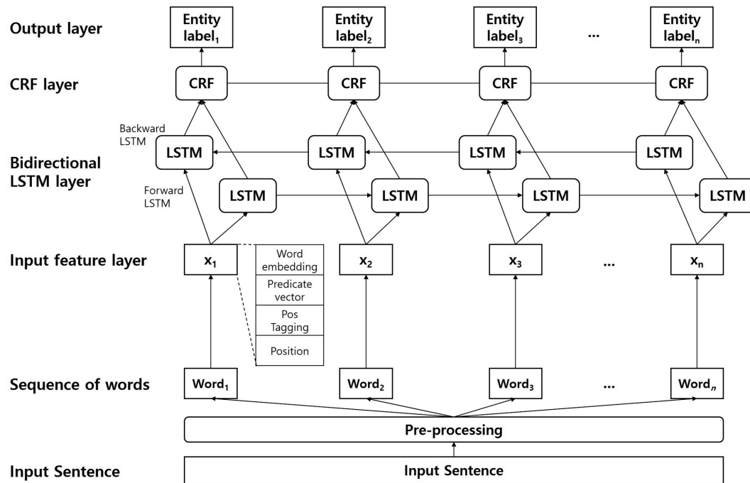
Figure 6: Deep learning-based semantic role labeling process.
