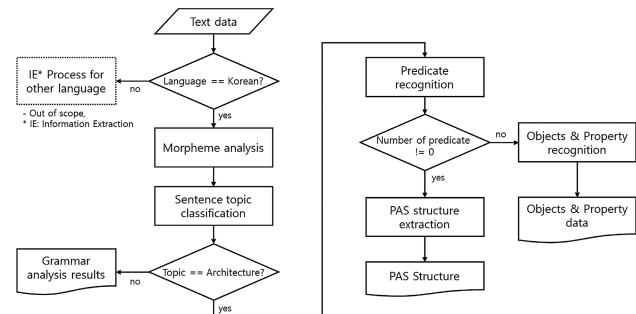
Figure 5: Deep learning and NLP-based building design PAS extraction process.
