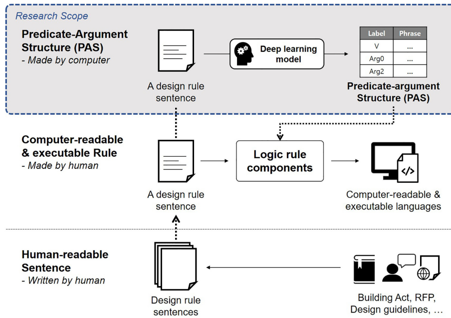
Figure 1: Overview of NLP-based regulatory information extraction for a building design rule-checking system.
