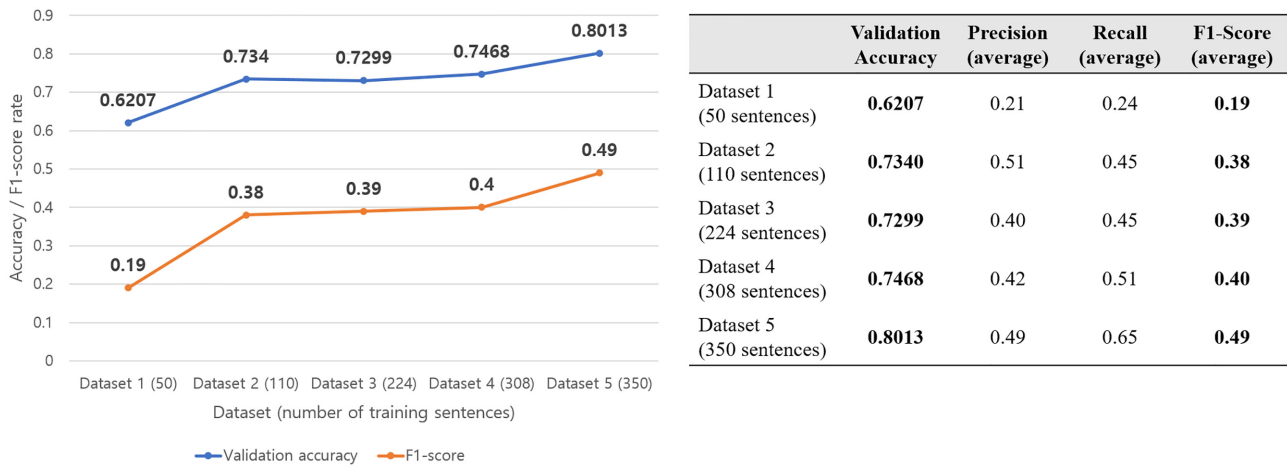
Figure 7: Validation accuracy and F1 score measurements by dataset.
