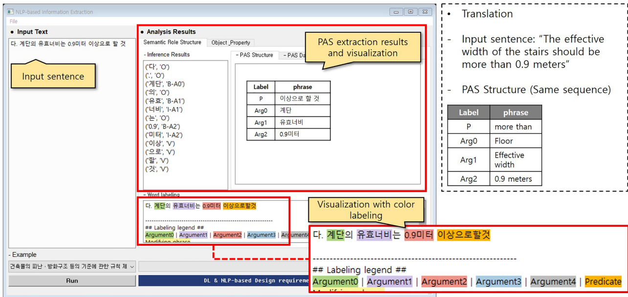
Figure 9: A snapshot of the GUI application prototype.
