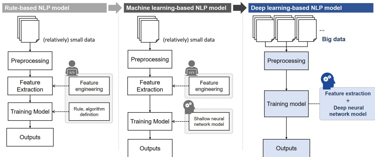
Figure 4: Comparison between classical NLP model and deep learning-based NLP model.
