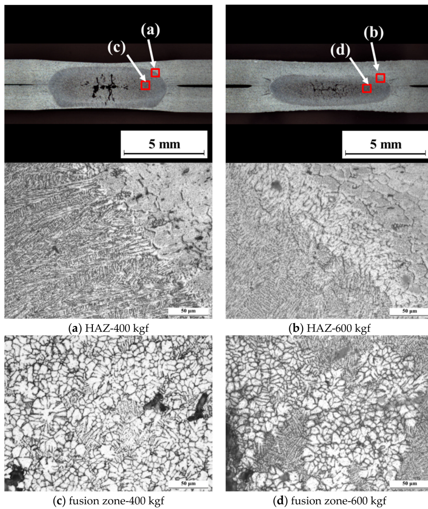
Figure 5. Microstructures of heat-affected zone (HAZ) and fusion zone obtained with the as-received electrode at electrode forces of 400 kgf and 600 kgf.
