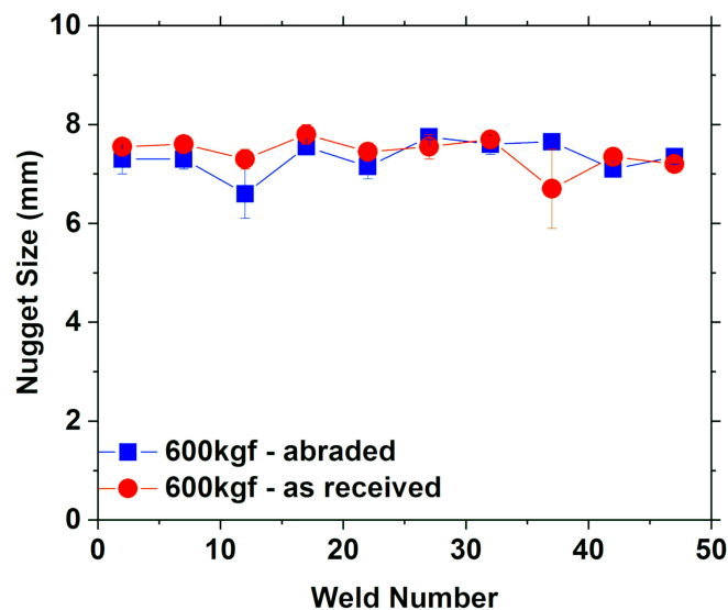
Figure 8. Measured nugget size during continuous RSW under the electrode force of 600 kgf.
