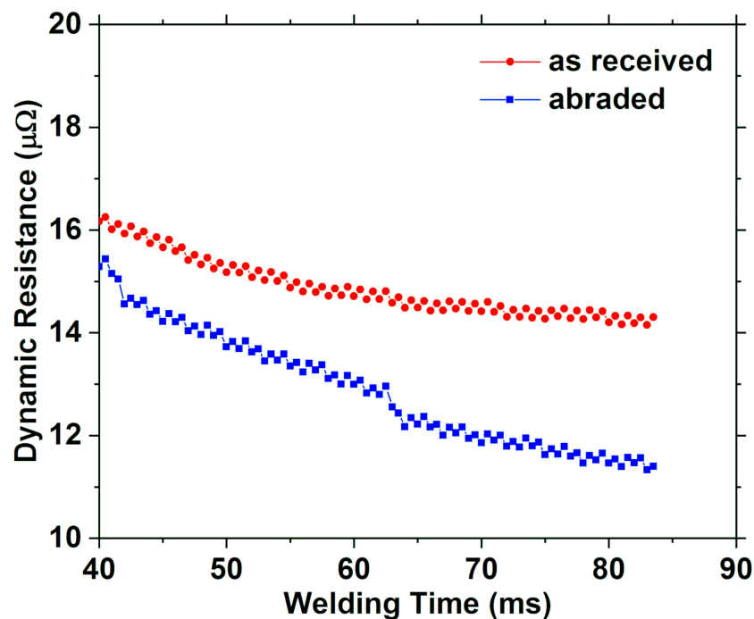
Figure 17. Measured dynamic resistance between base material and electrodes.
