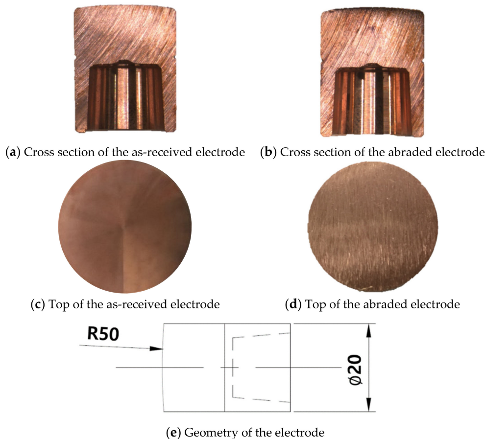
Figure 1. Configuration of the electrodes used in this study.
