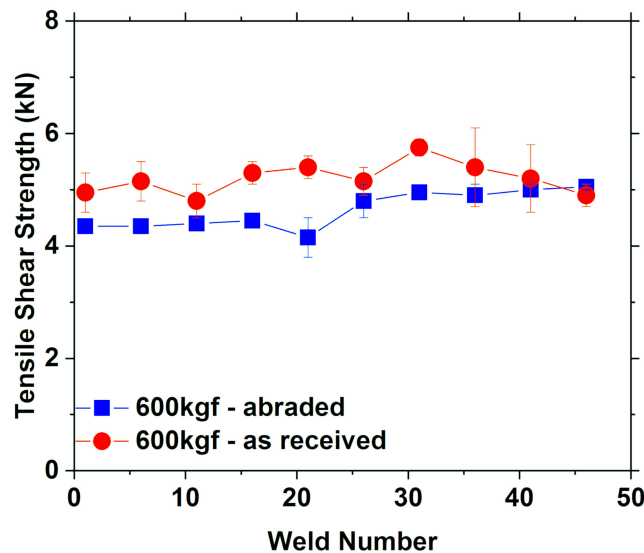
Figure 10. Measured tensile shear strength during continuous RSW under the electrode force of 600 kgf.
