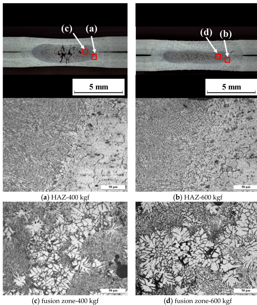
Figure 6. Microstructures of HAZ and fusion zone obtained with the abraded electrode at electrode forces of 400 kgf and 600 kgf.
