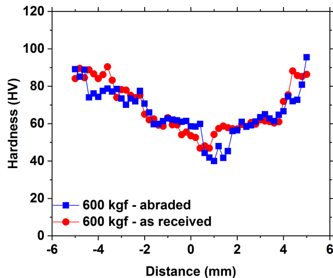
Figure 3. Measured hardness distribution of welds produced at the electrode force of 600 kgf.
