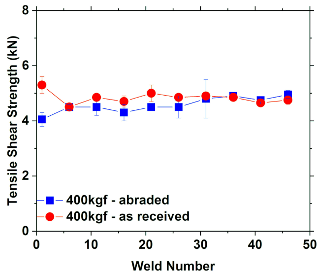
Figure 9. Measured tensile shear strength during continuous RSW under the electrode force of 400 kgf.
