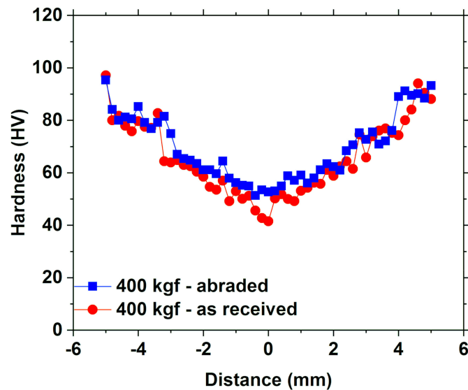
Figure 2. Measured hardness distribution of welds produced at the electrode force of 400 kgf.
