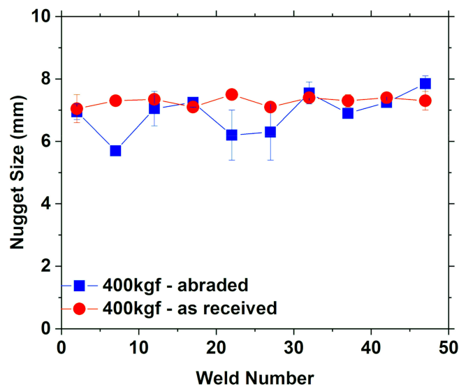
Figure 7. Measured nugget size during continuous resistance spot welding (RSW) under the electrode force of 400 kgf.
