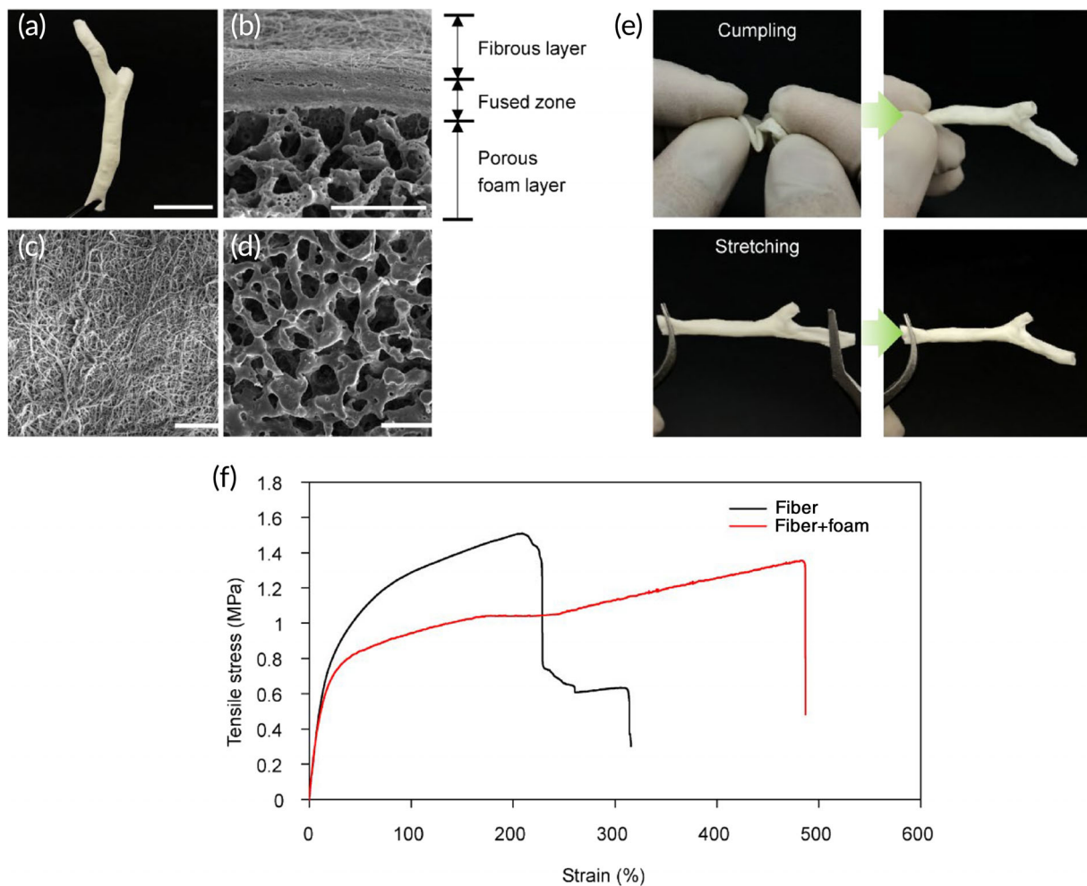
FIGURE 2 Characterization of 3D customized dual-layer tubular scaffold. (a) Overall shape of the final scaffold. (b) Representative scanning electron microscopy (SEM) image of cross section through dual layer scaffold. (c) SEM image of inner surface of fiber layer. (d) SEM image of outer surface of porous foam layer. (e) Manual resilience tests by harsh crumpling and stretching. (f) Tensile testing of 3D scaffolds engineered as a dual layer or fiber-only layer. Scale bars: 20 mm (a); 50 \mu m (b), 100 \mu m (c, d)
