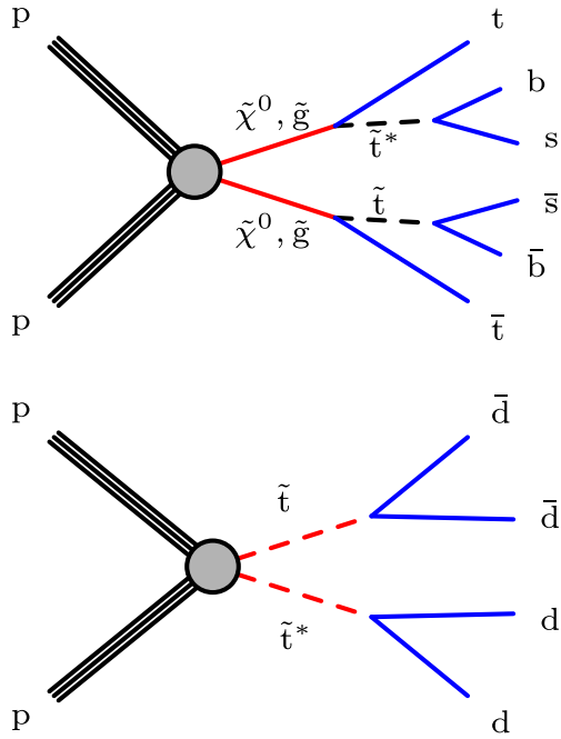
FIG. 1. Diagrams of the multijet signal model (upper) showing long-lived neutralinos ( \tilde{\chi}^0 ) or gluinos ( \tilde{g} ) decaying into top, bottom, and strange quarks via virtual top squarks ( \tilde{t} ), and the dijet signal model (lower) showing long-lived top and anti-top squarks decaying into two down-type quarks. In both cases, the long-lived particles are the LSPs in their respective models.
