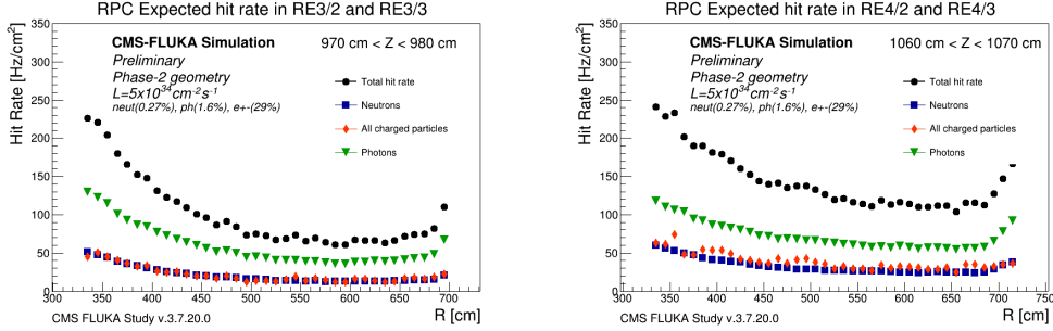
Figure 3. Averaged expected hit rates at an instantaneous luminosity of 5 \times 10^{34} \text{ cm}^{-2} \text{ s}^{-1} are shown in the figure. The plot on the left represents expectation for the RE3/2 and RE3/3 RPC, and on the right for RE4/2 and RE4/3. The second rings RE3/2 and RE4/2 start at R \sim 332 \text{ cm} and the third rings RE3/3 and RE4/3 at R \sim 503 \text{ cm} . Different colors depict the contributions from different particle types. Z is along the beam pipe and depicts the distance from the interaction point, and R is a distance from the beam pipe in radial direction.
