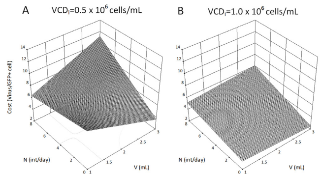
Figure 2: Fitted response surface model for virus cost per transduced cell due to variation of agitation cycles (N) and working volume (V) at (A) low seeding density (VCD) and (B) high seeding density
