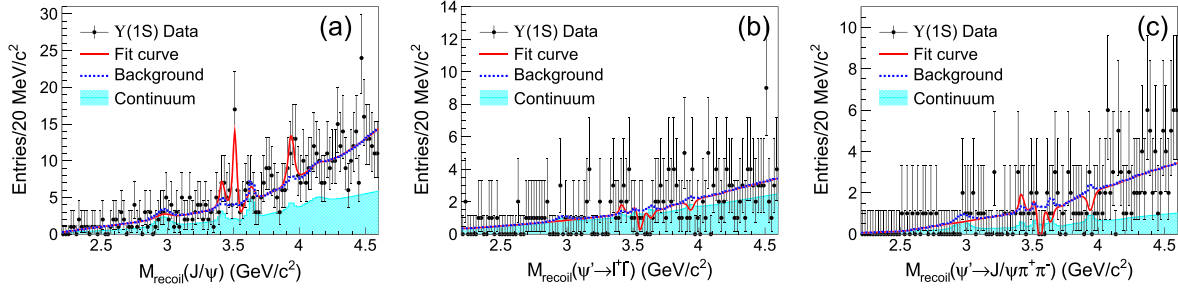
FIG. 3 (color online). Fit to the recoil mass spectra against the (a) J/\psi(\rightarrow \ell^+\ell^-) , (b) \psi'(\rightarrow \ell^+\ell^-) and (c) \psi'(\rightarrow J/\psi\pi^+\pi^-) in \Upsilon(1S) decays from data (points with error bars). The red solid curves are the nominal fits and the blue-dashed curves show the total background. The fitted normalized continuum contributions are represented by the cyan-shaded histograms.
