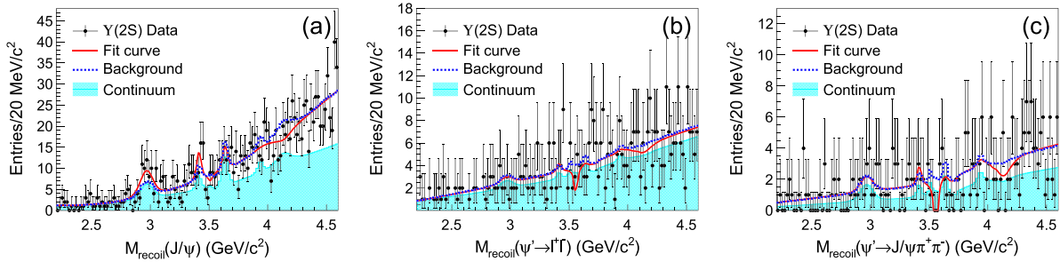
FIG. 4 (color online). Fit to the recoil mass spectra against (a) J/\psi(\rightarrow \ell^+\ell^-) , (b) \psi'(\rightarrow \ell^+\ell^-) and (c) \psi'(\rightarrow J/\psi\pi^+\pi^-) in \Upsilon(2S) decays from data (points with error bars). The representations of the curves and histograms in each graph match those in Fig. 3.
