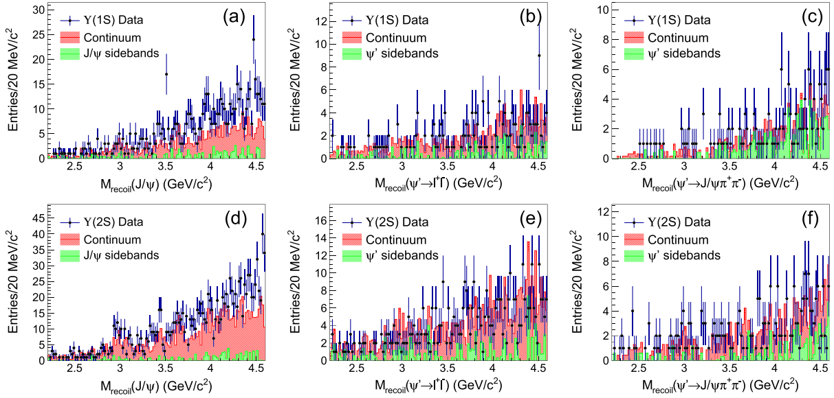
FIG. 2 (color online). Distributions of the recoil masses against the reconstructed J/\psi(\rightarrow \ell^+\ell^-) , \psi'(\rightarrow \ell^+\ell^-) , \psi'(\rightarrow J/\psi\pi^+\pi^-) within the J/\psi or \psi' mass signal regions from left to right. The upper and lower three graphs are for \Upsilon(1S) and \Upsilon(2S) decays, respectively. The red-shaded histograms are from the normalized continuum sample at \sqrt{s} = 10.52 GeV, and the green ones represent the scaled J/\psi(\psi') mass sideband backgrounds from \Upsilon decays.
