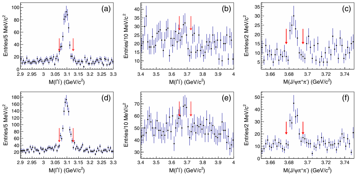
FIG. 1 (color online). Distributions of the invariant masses of J/\psi identified with lepton pairs and \psi' identified with both \ell^+\ell^- and J/\psi\pi^+\pi^- with the J/\psi(\psi') recoil mass within 2.2 \text{ GeV}/c^2 and 4.6 \text{ GeV}/c^2 from left to right. The upper and lower three graphs are for \Upsilon(1S) and \Upsilon(2S) decays, respectively. The arrows show the signal regions of J/\psi or \psi' masses.
